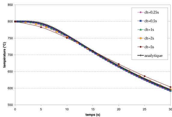
(e) Evolution thermique Gdimp z = 20mm
