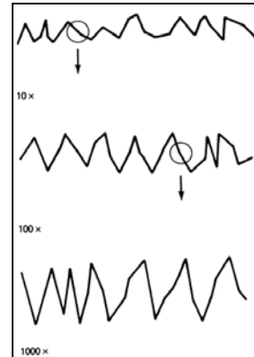
Figure 4.1. Fractale auto affine
