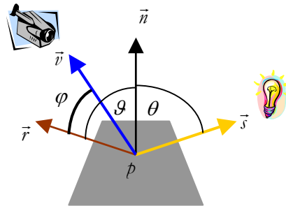
Figure App-1. The reflected light that reaches the camera lens depends on the direction of the normal to the surface ( \vec{n} ) the vector from the studied point to the light source ( \vec{s} ) and the vector from the point to the camera lens ( \vec{v} ). \psi = \varphi for perfectly specular reflections.
