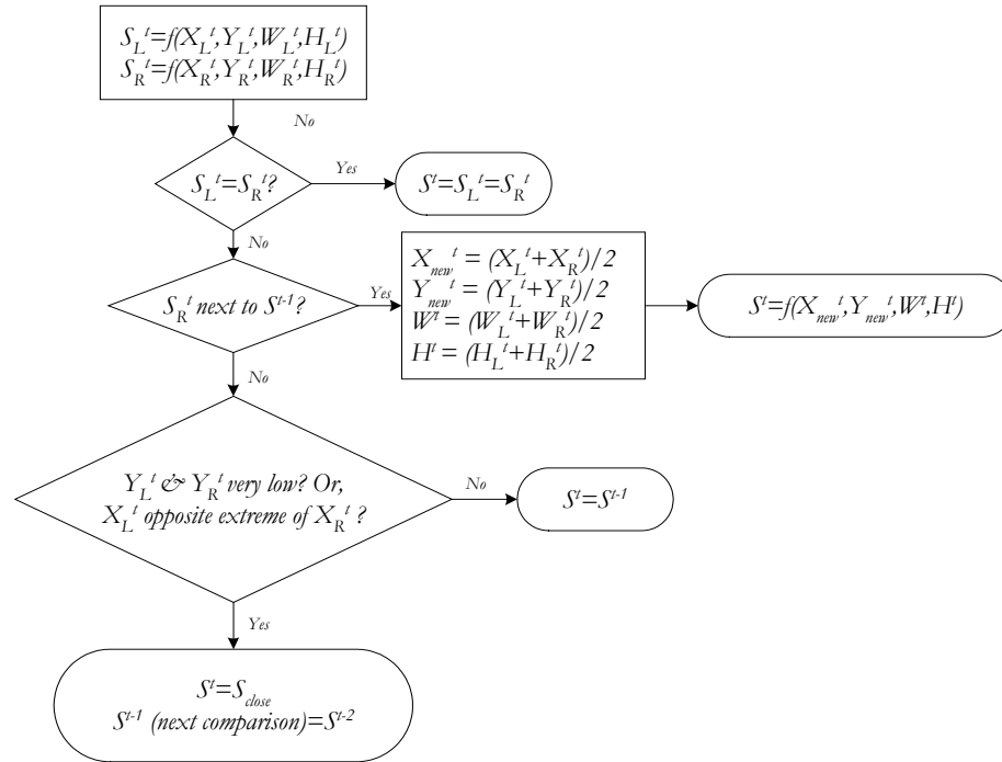
Figure IV-3. The analyzed results of each eye feature are filtered through this Temporal Diagram. Current eye states S_L^t and S_R^t are contrasted to obtain a common state for both eyes: S^t . Since the state S_{close} does not have any physical information about the pupil location, it is ignored for future analysis in the temporal chain. The starting state is fixed with the X, Y of the eyes in their neutral position
