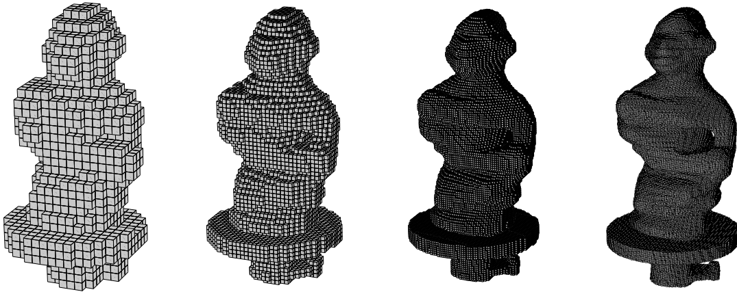
Figure 2.7: Octree construction of a visual hull. From left to right, the level of detail ranges from 5 to 8 depth levels.
