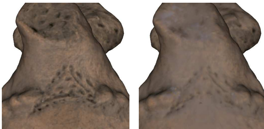
Figure 3.47: Comparison between using the two color sequences to generate the texture map (left) or using only the first color sequence (right).
