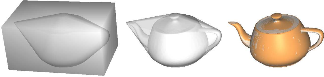
Figure 2.2: Different object initializations. From left to right: bounding box+convex hull, convex hull+visual hull, visual hull + real object.
