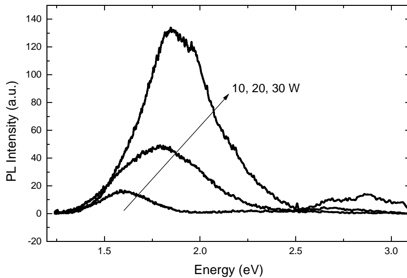
Fig. 5.23. Room temperature PL spectra of pm-Si_{1-x}C_x:H films deposited at 3500 mTorr with a substrate temperature of 200 °C for three values of the RF power. The samples were excited using a HeCd laser at 325 nm (3.8 eV).
