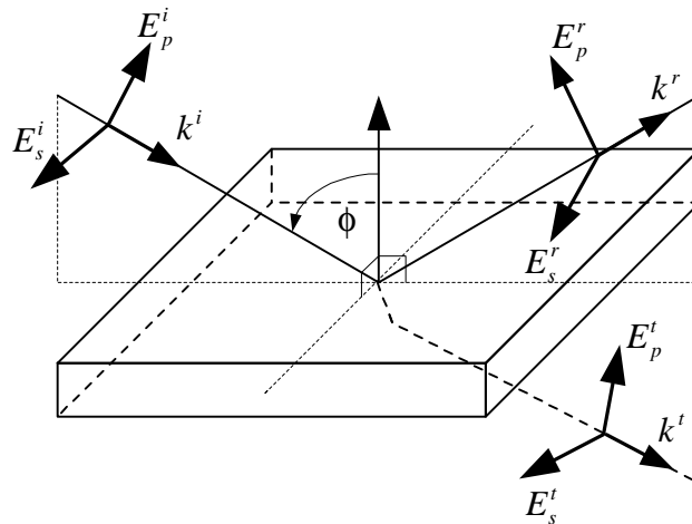
Fig. 2.9. Schematic diagram of incident, reflected and transmitted light on thin slab
