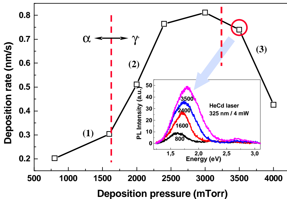
Fig. 4.3. A typical pressure dependence curve of the deposition rate for pm-Si_{1-x}C_x:H at 200 °C and RF power of 20 W ( 0.21 \text{ W/cm}^2 ). The inset shows the effect of deposition pressure on the PL spectra of pm-Si_{1-x}C_x:H thin films deposited in the same conditions.
