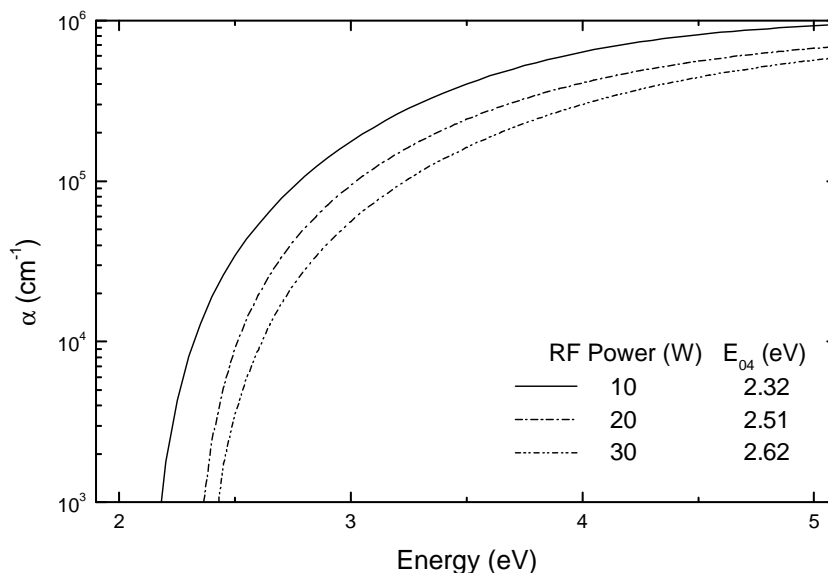
Fig. 5.11. The effect of RF power on the absorption coefficient of pm\text{-Si}_{1-x}\text{C}_x\text{:H} films deposited at 200^\circ\text{C} and 3500 mTorr.
