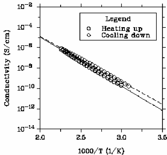
Fig. 2.24. Temperature dependence of the dark conductivity for a pm-Si_{1-x}C_x:H film and the fitting results according to the Arrhenius model for heating up and cooling down process.
