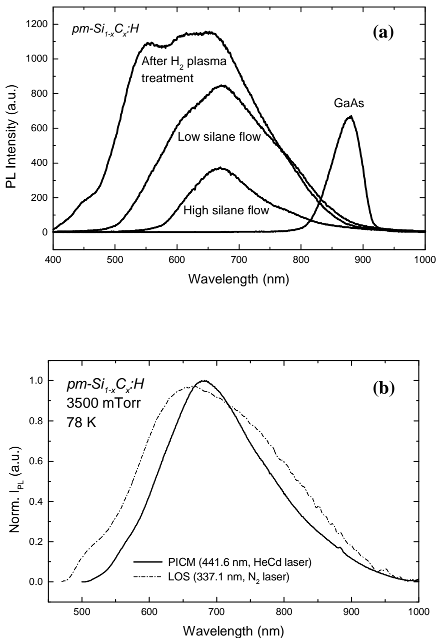
Fig. 2.18. a) Typical PL spectra for pm-Si_{1-x}C_x:H samples with GaAs PL emission peak as a reference. All the samples were measured at ambient temperature under the same measurement conditions ( \lambda_{exc.} = 325 nm). b) Comparison of PL spectra of the same sample measured at 78 K with the PL setup at PICM (full line) and at LOS (dash-dot line).
