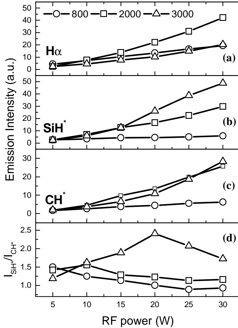
Fig. 4.16. The evolution of optical emission intensity of a) H\alpha , b) SiH^* , c) CH^* lines and d) emission intensity ratio between SiH^* and CH^* lines as functions of RF power at various pressures.
