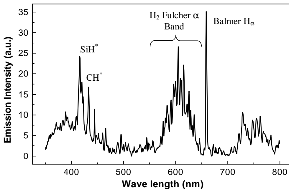
Fig. 4.10. Optical emission spectrum from a \text{SiH}_4\text{-CH}_4\text{-H}_2 glow discharge with an RF power of 0.21 \text{ W/cm}^2 at 1600 mTorr. Both electrodes were heated at 200 \text{ }^\circ\text{C} .
