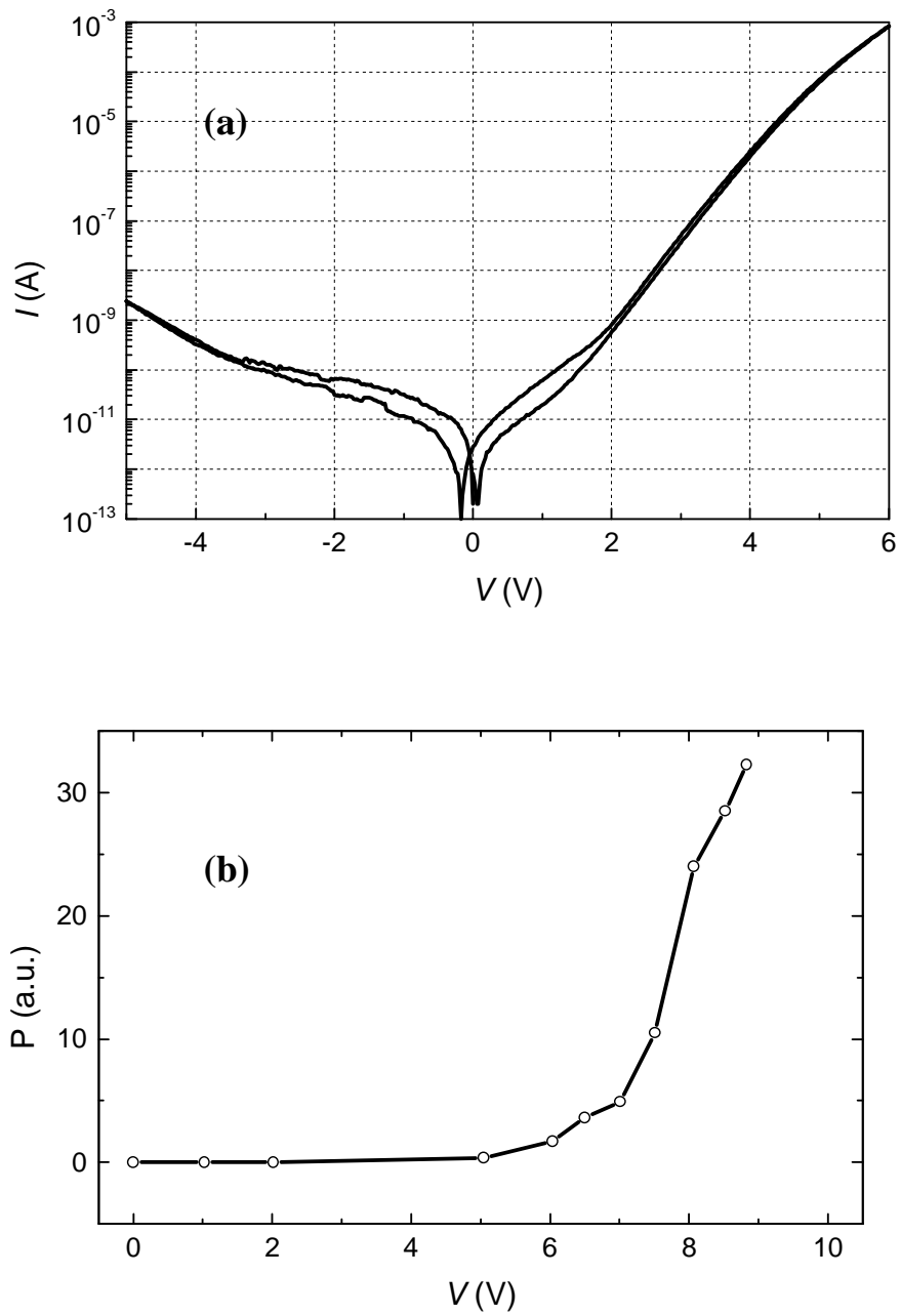
Fig. B.1. (a) The I-V characteristics of pm\text{-Si}_{1-x}\text{C}_x\text{:H} EL p\text{-}i\text{-}n diode for samples with structure as mentioned in Fig. 2.16b. (b) The emitted power as function the applied voltage for the same electroluminescent diode.
