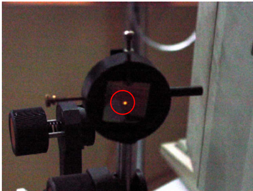
Fig. 1.1. Red light emission of a pm-Si 1-x C x :H film excited by a 4 mW HeCd laser at 325 nm.
