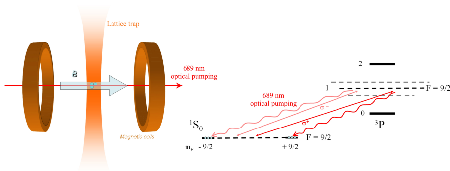
Figure 2.7: Right: The relevant transitions of the optical pumping scheme. The polarization of the 689 nm laser is alternated between \sigma^+ and \sigma^- between cycles. Left: A sketch of the experimental realization. The blue circles represent atoms.
