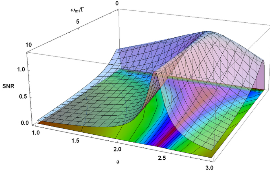
Figure 3.5: The signal-to-noise ratio in units of 2C_0\sqrt{\frac{\eta S I_{\text{sat}} n_\gamma}{\hbar \omega_0 \Gamma}} as a function of modulation depth a in radians and modulation frequency in units of the line width, \omega_m/\Gamma .
