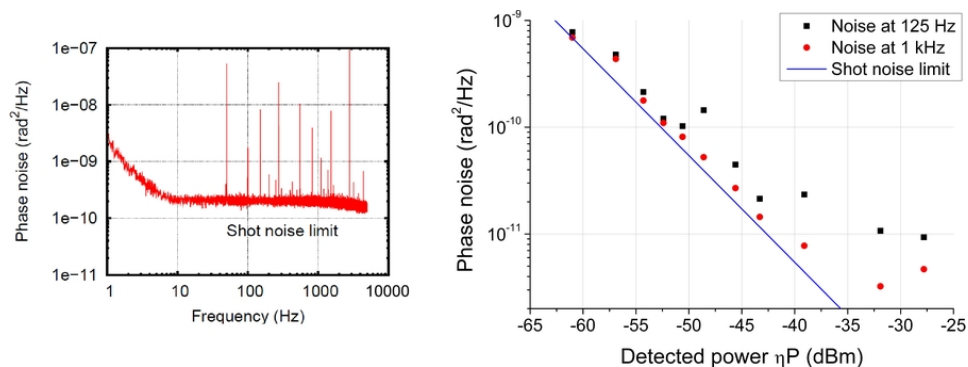
Figure 3.6: The power spectral density of the detection noise \left(\frac{1}{2}\sqrt{\langle\delta\varphi_1^2\rangle + \langle\delta\varphi_{-1}^2\rangle}\right) . Left: The phase noise spectrum for a typical detected power \eta P = 5 nW. The signal is shot noise limited above 10 Hz. Right: The phase noise at frequencies 125 Hz and 1 kHz for different detected powers. The blue line shows the shot noise limit calculated from (3.33) with no adjustable parameters.
