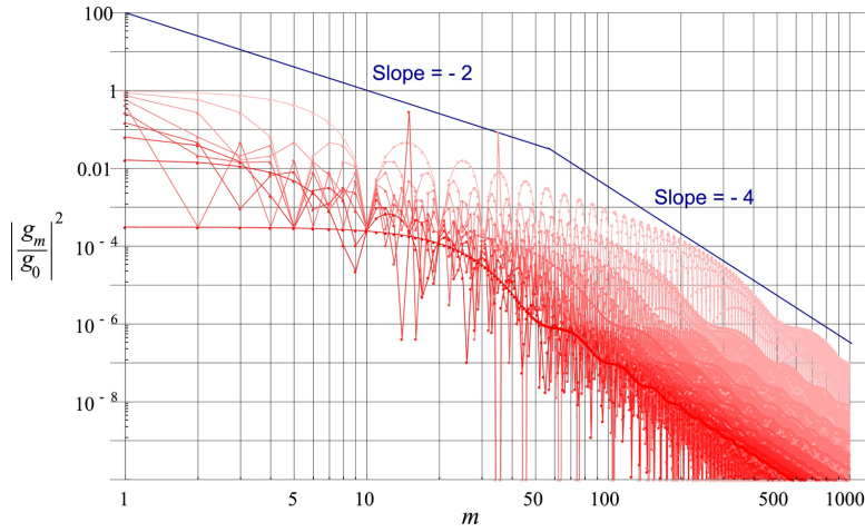
Figure 5.3: The normalized Fourier components \left|\frac{g_m}{g_0}\right|^2 for Ramsey interrogation with \Omega_0\tau_p = \pi/2 and \tau_p/T = 0.025 for duty cycles d = 0.1 to 1 from light to dark red with d = 1 being the darkest.
