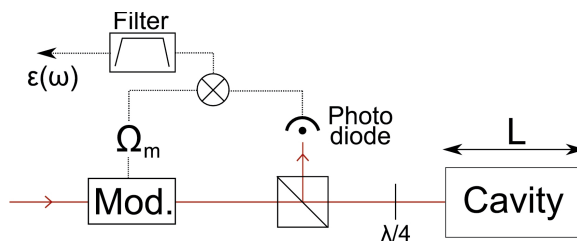
Figure 4.1: A sketch of the Pound-Drever-Hall setup for locking to a cavity. \Omega_m is the modulation frequency and \varepsilon(\omega) is the error signal.
