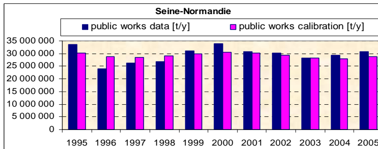
Figure 26: Calibration results for the demand of public works of Seine-Normandie
