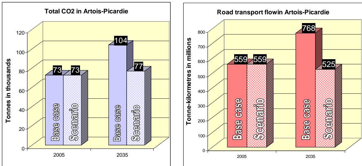
Figure 67: Total CO2 emissions and road transport flow in the scenario of recycling increase in Artois-Picardie
