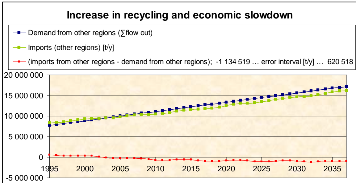
Figure 70: Recycling and economic slowdown consolidation: flow balance
