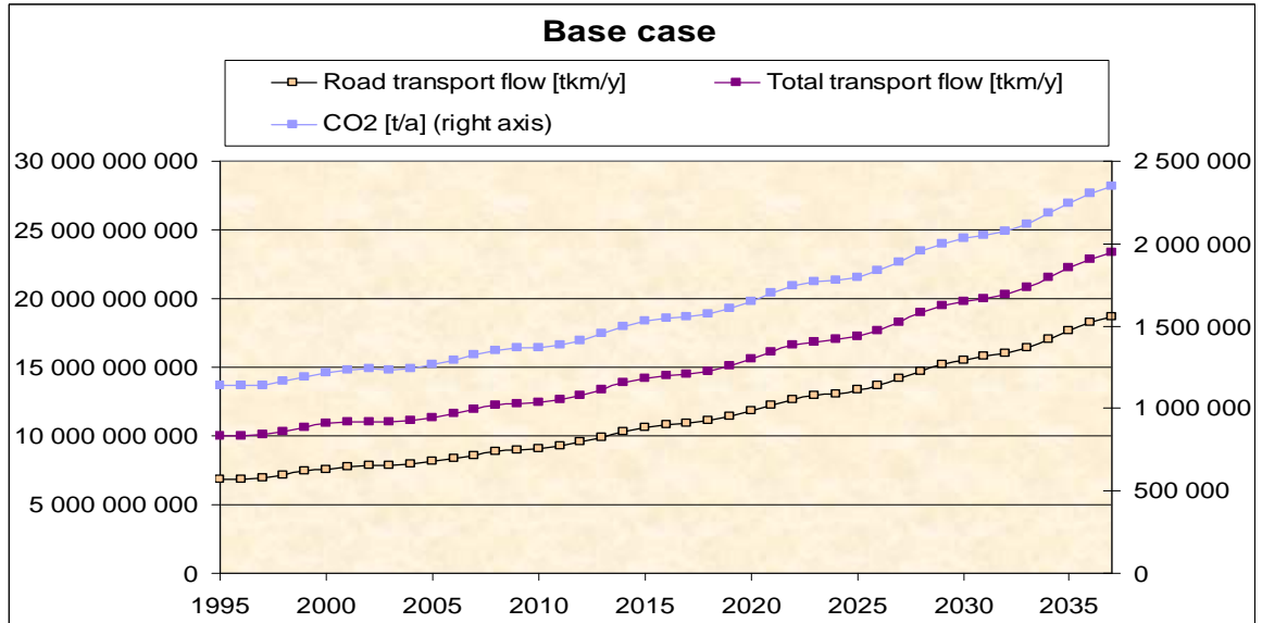
Figure 43: Base case consolidation: impacts
