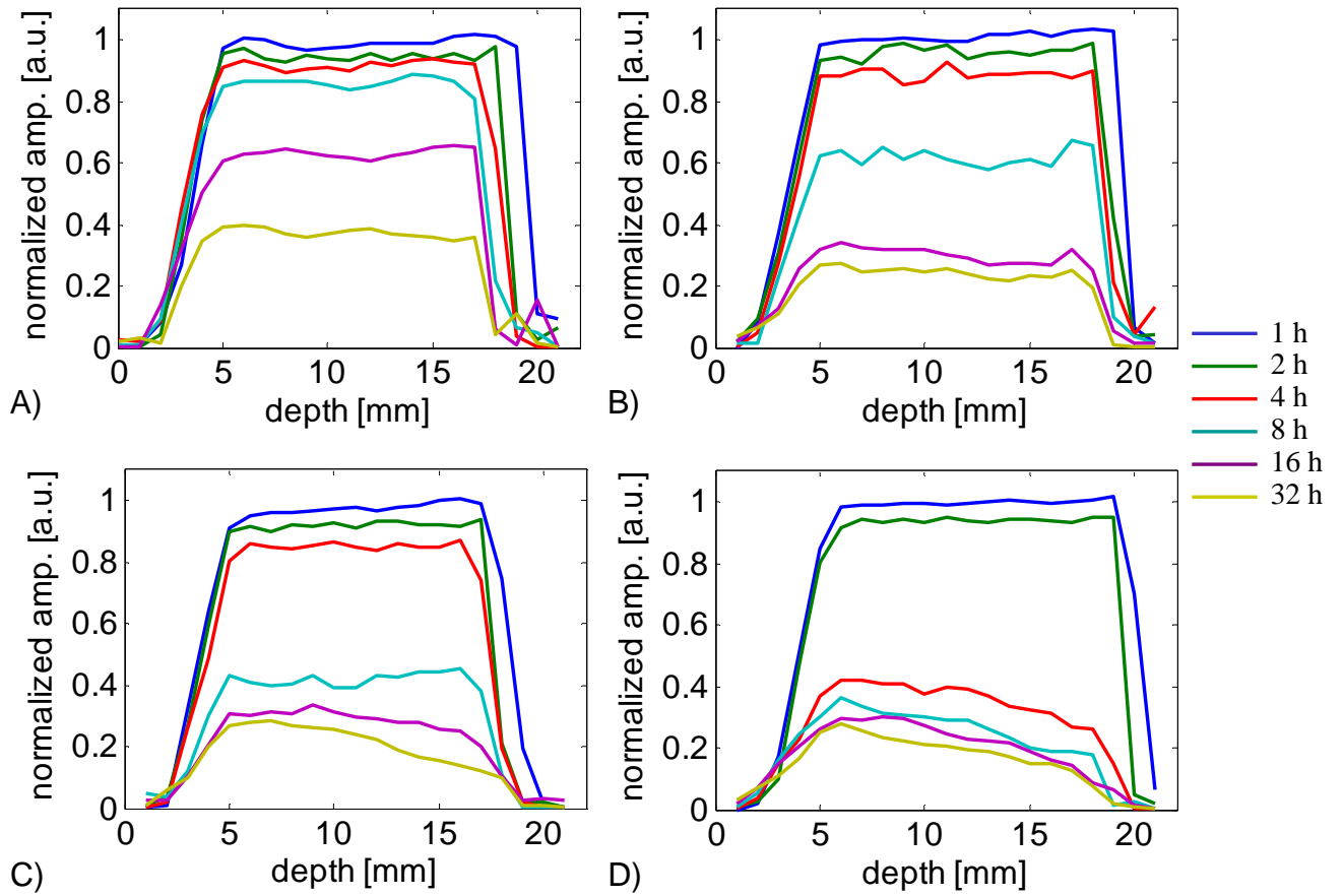
Figure 4.14: Profiles obtained using the NMR-MOUSE™ at various hydrating times and various temperatures: (A) 5 °C, (B) 20 °C, (C) 25 °C and (D) 35 °C on a white cement paste hydrated with a w/c ratio equal to 0.4. The profiles were measured over a range of 22 mm with a step of 1 mm. For each temperature, a profile was measured at exponentially spaced intervals of time: 1 h, 2 h, 4 h, 8 h, 16 h and 32 h, corresponding to the 6 downwards solid lines (blue, green, red, cyan, purple and yellow) of each plot. For each point of the profile, a CPMG detection train with an echo time of 140 \mu s was applied. Until a drying time of 4 h, 128 echoes were used in the CPMG train, the recycle delay was 1 s and the number of scans 48, leading to a total experimental time of 18 min. Beyond 4 h, the number of echoes was changed to 64, the recycle delay to 0.7 s and the number of scans to 128, so the total experimental time was 33 min. The amplitudes reported in the plots are the amplitudes obtained from a single exponential fit of the CPMG decay.
