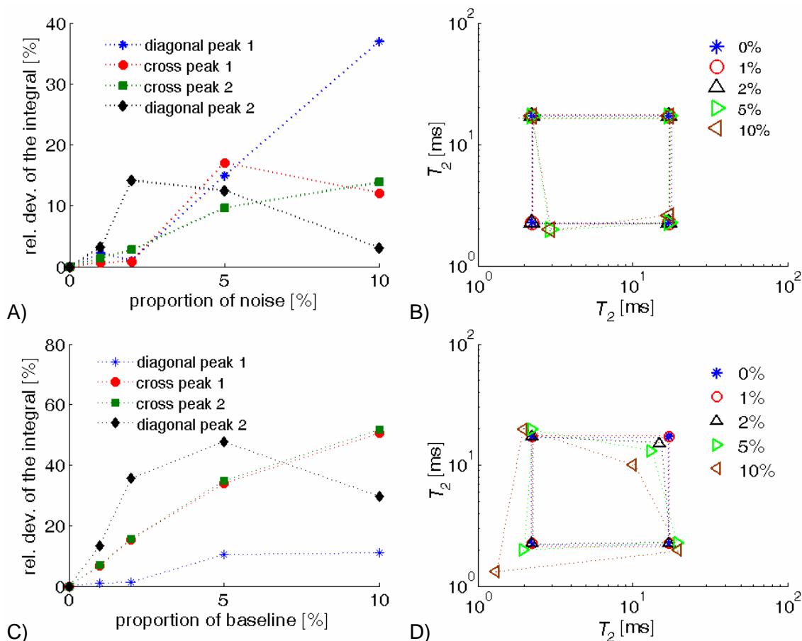
Figure 5.10: Effects of the noise (A and B) and baseline offset (C and D) on the peak intensities (A and C) and peak coordinates (B and D). The relative deviation of the integrals from the value in the absence of noise is given in percent. The baseline offset is specified relative to the maximum value of the original time-domain 2D data set.
