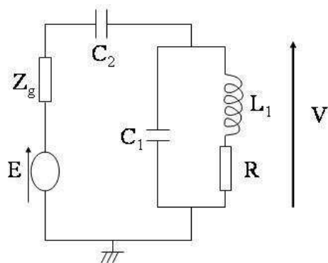
Figure 1.6: Parallel RLC circuit in series with a matching capacitor (so-called "tank" circuit).
