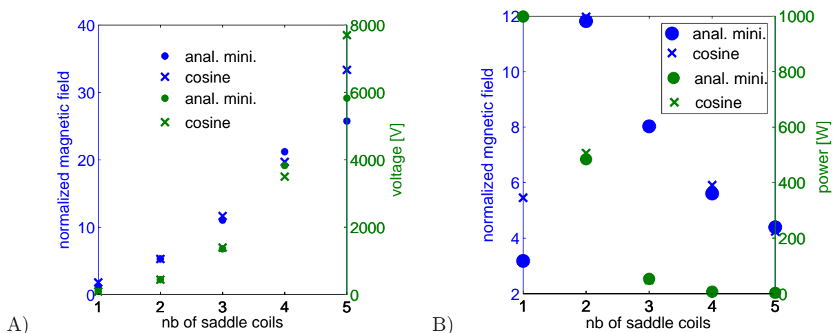
Figure 1.18: A) Magnetic field generated by multiple saddle coils and voltage at the output of the tuning capacitor assuming an input power of 100 W. B) Magnetic field generated by multiple saddle coils and input power assuming the voltage at the output of the tuning capacitor is 1 kV.
