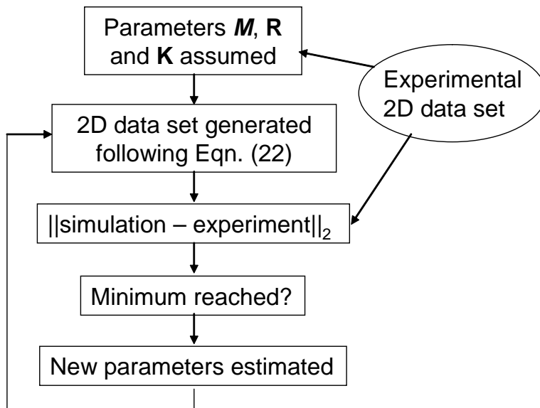
Figure 5.13: Flowchart demonstrating the procedure used to fit the experimental data. At each iteration, the simplex algorithm is used to estimate a new set of parameters minimizing the least-squares misfit of measured and experimental data points.
