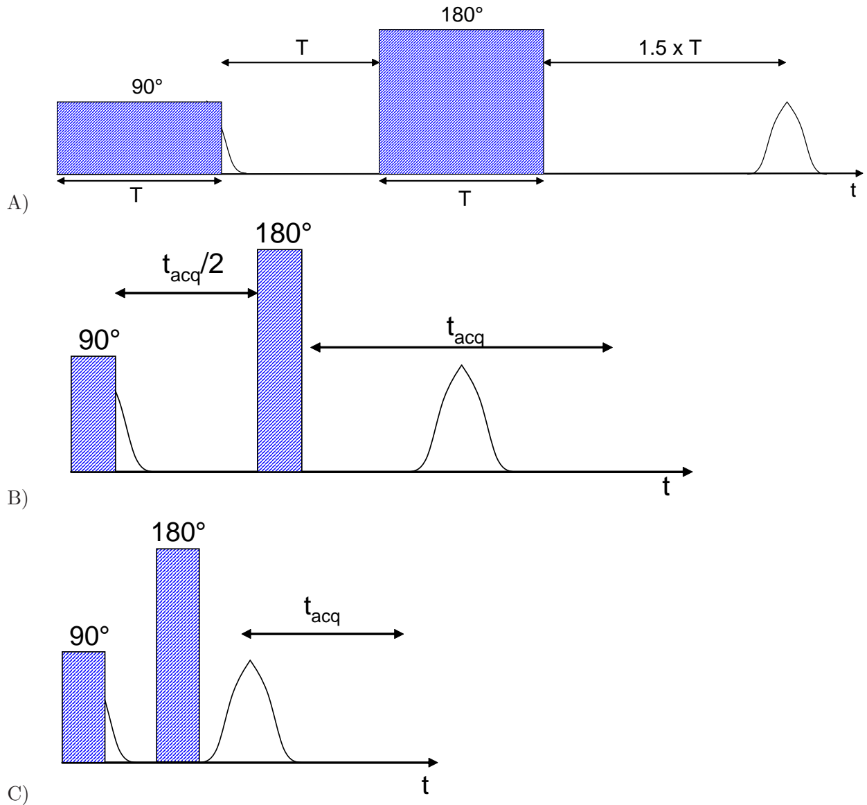
Figure 2.22: A) Pulse sequence for thin slice selection. B) Pulse sequence for long acquisition time. C) Pulse sequence for half echo recording.
