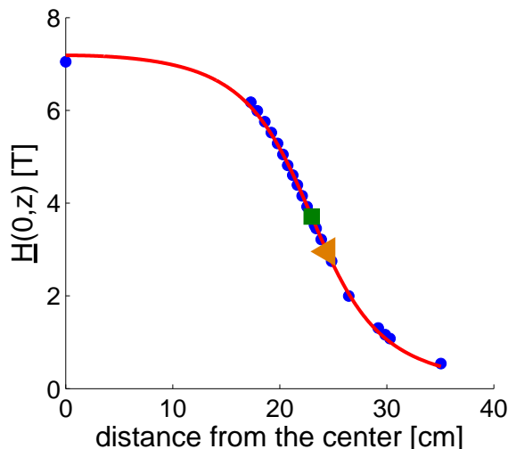
Figure 2.11: Magnetic field along the z axis of the superconducting magnet (points) and fitting with a solenoid model (line). The square represents the inflexion point and the triangle the theoretical position of the STRAFI plane of the solenoid model.
