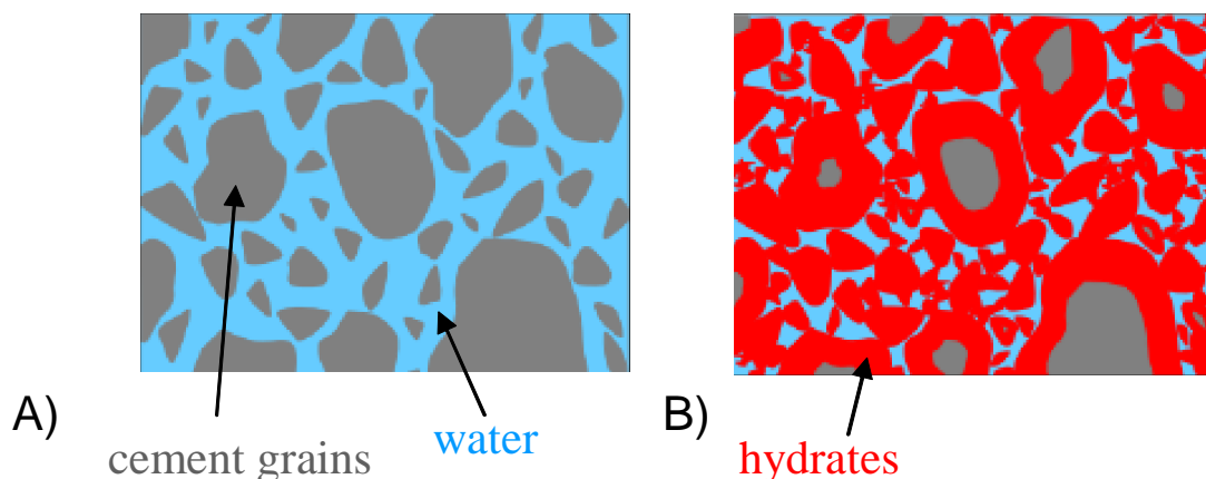
Figure 4.2: Sketch of cement grains before the hydration (A) and after (B). The outer layer of the grains dissolves, reacts with water and reprecipitates around the grain increasing its size and brings grains into contact.
