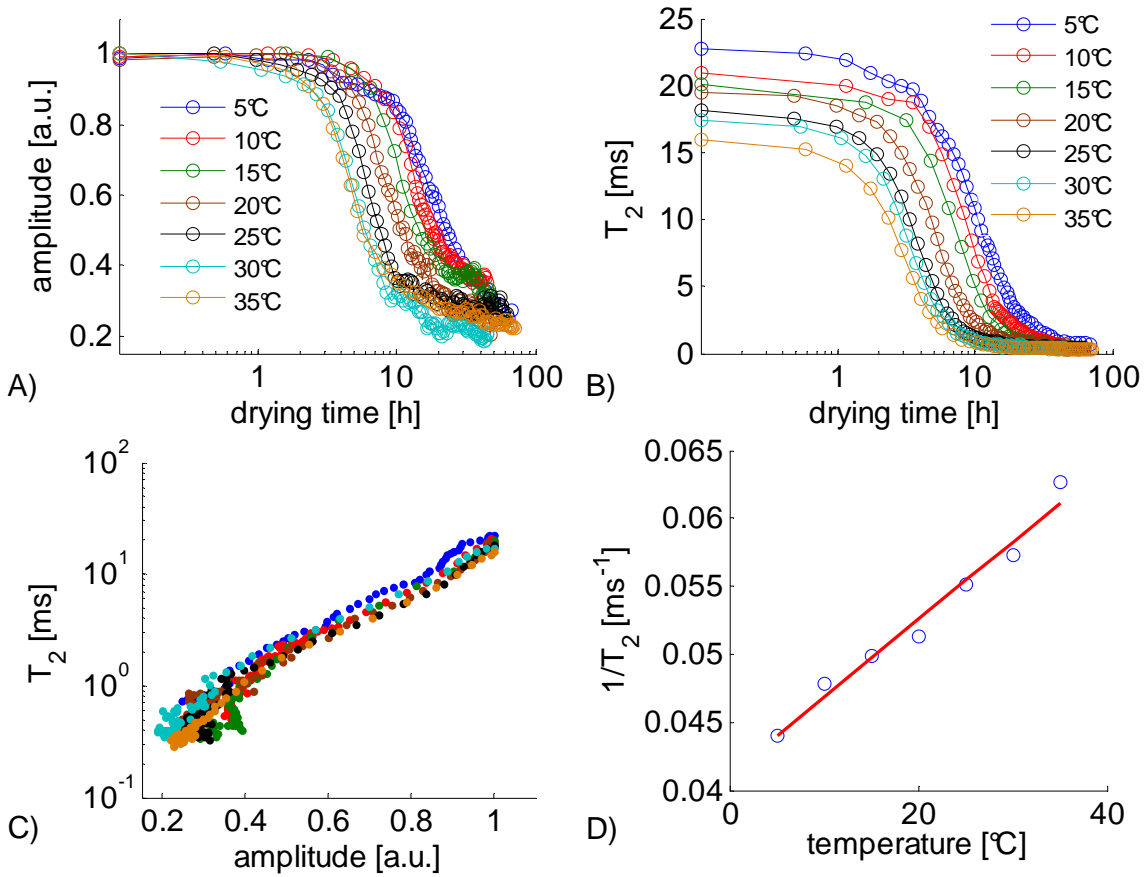
Figure 4.15: Amplitudes and T_2 relaxation rates as function of the drying time measured with the NMR-MOUSE™ at a single height in a sample of white cement ( w/c = 0.4 ). For these measurements, a CPMG detection train with an echo time of 140 \mu\text{s} was used. Until a drying time of 4 h, 128 echoes were used in the CPMG train, the recycle delay was 1 s and the number of scans 256, leading to a total experimental time of 4 min. Beyond 4 h, the number of echoes was changed to 64, the recycle delay to 0.7 s, and the number of scans to 512, so the total experimental time was 6 min. The amplitudes and T_2 's reported in the plots are obtained from single exponential fits of the CPMG decays. A) Evolution of the amplitudes versus the hydration time at various temperatures. B) Evolution of T_2 's versus the hydration time at various temperatures. C) Correlation between amplitudes and T_2 's at various temperatures. D) Correlation between the T_2 's measured at the initial drying time and the temperature.
