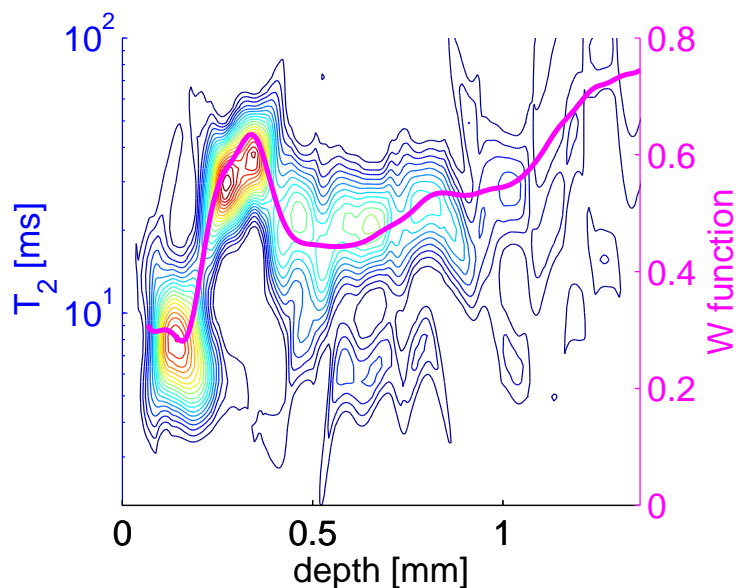
Figure 3.19: Depth-relaxation map of the skin tissue of the palm of the hand. The purple line corresponds to the w function (Eq. (3.19)). For the present T_2 distribution map 340 echoes were collected in the CPMG detection train where for each echo 128 complex points were acquired with a dwell time of 2 \mu\text{s} which sets a resolution of 50 \mu\text{m} . Using 2048 scans and a repetition time of 300 ms the total experimental time was 10 minutes. The w parameter was measured using 128 scans in 38 s.
