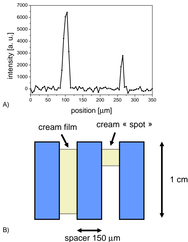
Figure 2.18: A) Step by step ( 5\ \mu\text{m} step) profile of a bilayer phantom two cream films separated by a 150\ \mu\text{m} glass plate. The NMR sequence is a CPMG detection train of 512 echoes with an echo time of 49\ \mu\text{s} . The repetition time was 0.5\ \text{s} and 64 scans were accumulated for each of the 70 points of the profile leading to a total experimental time of 37 min. B) Schematic (not to scale) of the bilayer phantom profiled in (A). The first film is 1\ \text{cm} wide.
