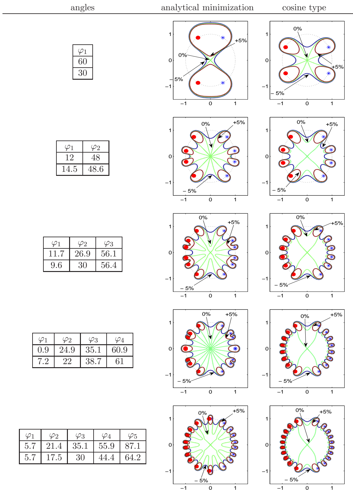
Figure 1.14: Angles allowing the optimum field homogeneity versus the number of saddle coils according the analytical minimization of Javelot (upper values) or an imitation of the cosine distribution (lower values). On the right, are displayed the corresponding field maps. The isofield lines are at \pm 5\%
