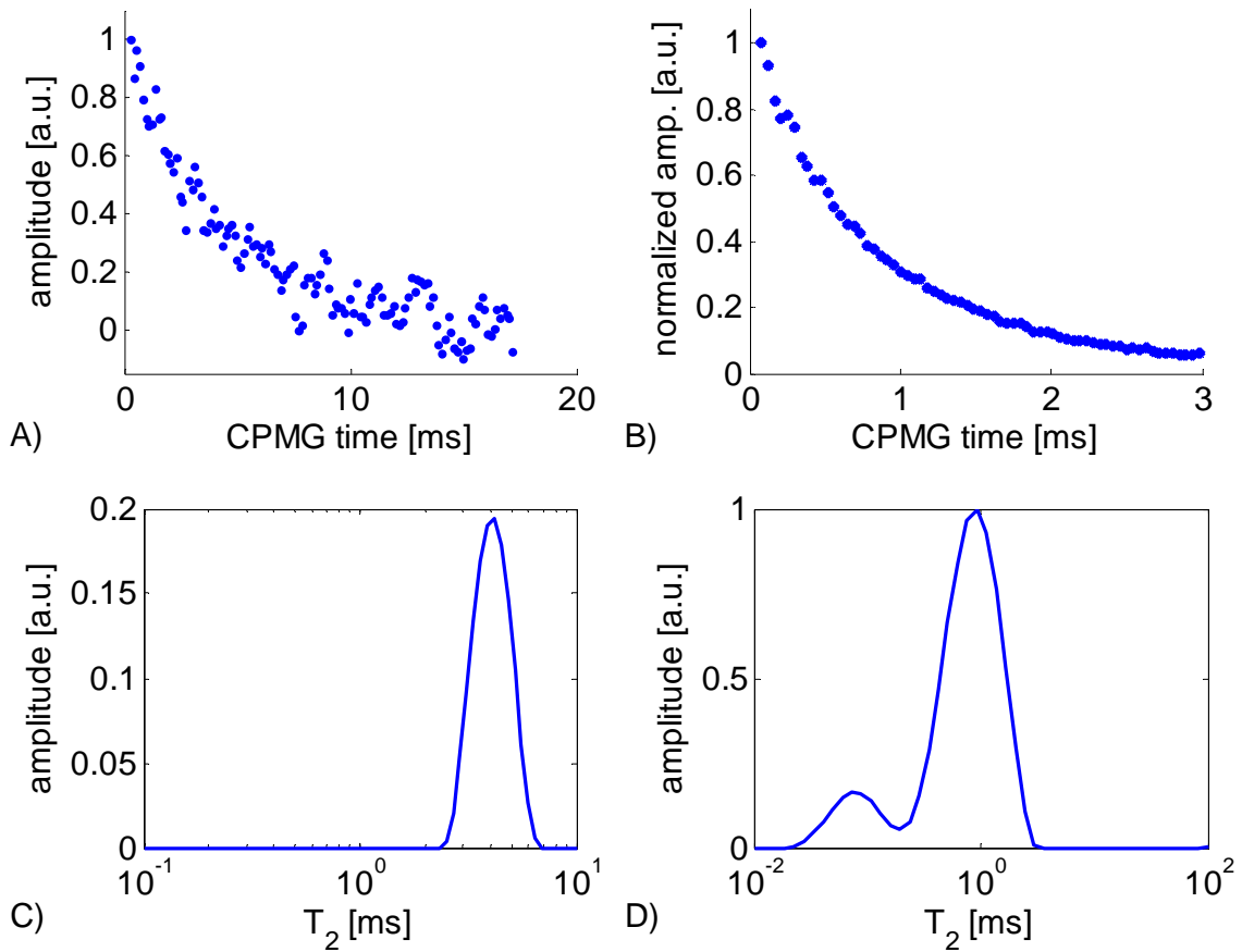
Figure 4.10: CPMG decays and associated T_2 distributions of white cement prepared with a ratio water/cement equal to 0.4 after 8 hours of drying. A) CPMG decay obtained using the NMR-MOUSE™. The echo time was set to 140 \mu\text{s} and the number of echoes to 128. The repetition time was 1 s. and the number of scans 512. This led to an experimental time of about 8.5 minutes. B) CPMG decay obtained using STRAFI. The echo time was 40 \mu\text{s} and the number of echoes 400. Here are displayed only the first 64 echoes. The repetition time was 1 s. and the number of scans is 512, leading to an experimental time of 8.5 min. C) T_2 distribution obtained from the ILT of the CPMG decay displayed on A). D) T_2 distribution obtained from the ILT of the CPMG decay displayed on B).
