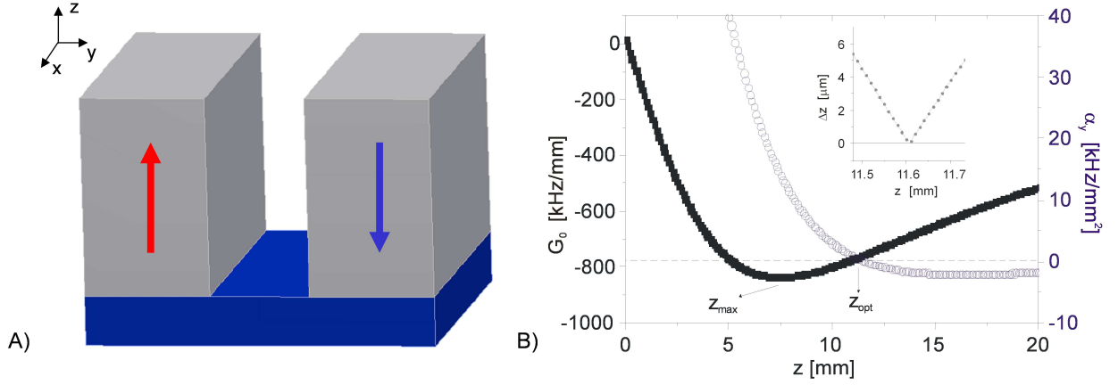
Figure 3.6: A) Sketch of a U-shaped magnet. Magnet blocks of SmCo magnetic material were used with dimensions of 140 \times 57 \times 80 \text{ mm}^3 . Setting the central gap g_y = 16 \text{ mm} a magnetic field of 0.42 \text{ T} was generated at the working depth ( z_{\text{opt}} ). B) Coefficients characterizing the most important field inhomogeneities of the U-shaped magnet as a function of the depth. The left ordinate shows the gradient G_0 while the right ordinate measures the second derivative of the field \alpha_y along the lateral direction y . Inset: upper bound for the resolution \Delta z calculated using Eq. (3.4). For each depth the G_0 value corresponds to the curve of solid squares and \Delta B = \alpha_y \cdot R^2 with \alpha_y obtained from the open circles and R = 5 \text{ mm} .
