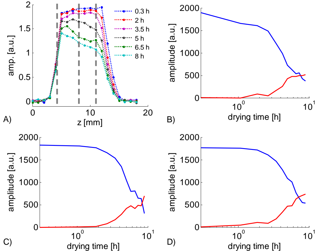
Figure 4.12: A) Profiles measured by STRAFI at various hydration time following the preparation of a sample of white cement ( w/c = 0.4 ) at 25^\circ\text{C} and 30\%rH . These profiles were measured using a CPMG detection train with an echo time of 40 \mu\text{s} . For the profiles, only the first echo was processed. The recycling delay was 1 s and the number of scans 64 in order to complete the 19 points of the profile in 20 min. The vertical grey dotted lines correspond to the position where a double exponential fit was performed. The amplitude of the long T_2 (blue solid line) and short T_2 (red solid line) versus the hydration time are exhibited in plots (B), (C) and (D).
