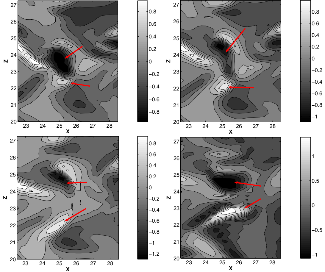
Figure 5.9: Sequence of figures showing the formation of streamwise vortices. The isocontours of the vorticity \omega_x are reported. From left to right and top to bottom: (a) t = 5 , (b) t = 7 , (c) t = 12 , (d) t = 17 . The two patches with positive and negative values of \omega_x are elongated in the streamwise direction and form two counter-rotating vortices.
