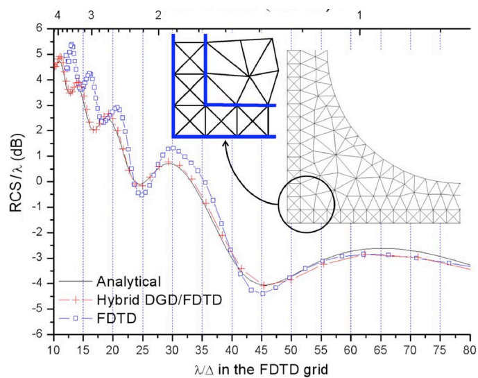
FIGURE 3.4 – Couplage de schémas 2D DG/DF - Garcia et al. [20]
