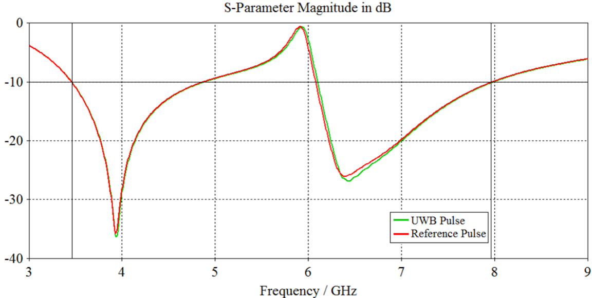
Fig. 4.19 – Return loss for the monopole antenna with CSRR filter inserted in the conductor patch, green curve antenna excited with UWB pulse and red curve Gaussian pulse.
