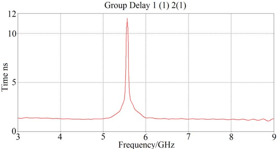
Fig. 4.20 – Group delay from two monopole antenna with CSRR filter inserted in the conductor patch.
