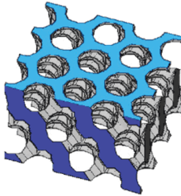
Fig. 2.13 – The first photonic crystal with a complete band gap [19].
