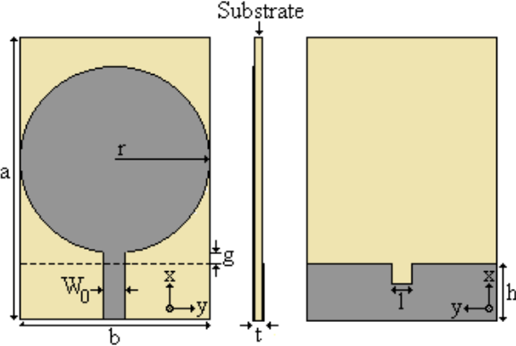
Fig. 4.4 – Circular monopole antenna with improved ground plane, where the gray region denotes a conductor material.
