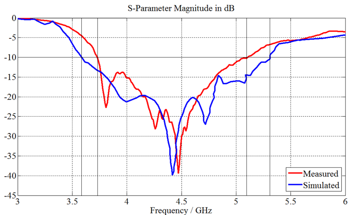
Fig. 6.11 – Return loss for the Fabry-Pérot suspended U-slot antenna.
