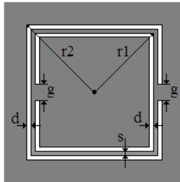
Fig. 4.22 – CSRR geometries. The gray region denotes a conductor material.
