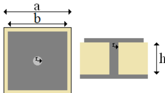
Fig. 5.4 – HIS unit cell superior view on the left and transversal cut on the right.
