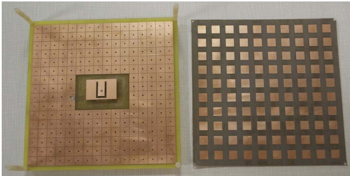
Fig. 6.9 – Constructed Fabry-Pérot suspended U-slot antenna.
