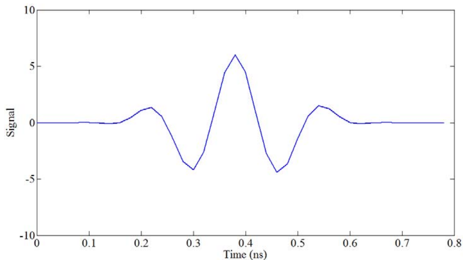
Fig. 4.18 – FCC pulse.
