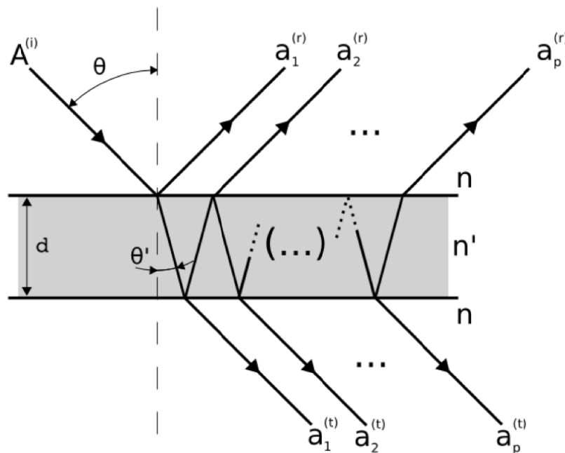
Fig. 6.2 – Graphical representation of a plane light wave with amplitude A^{(i)} focusing on a plate with flat and parallel surfaces. The n th reflected beam is represented by a_p^{(r)} while the n th transmitted beam is represented by a_p^{(t)} .
