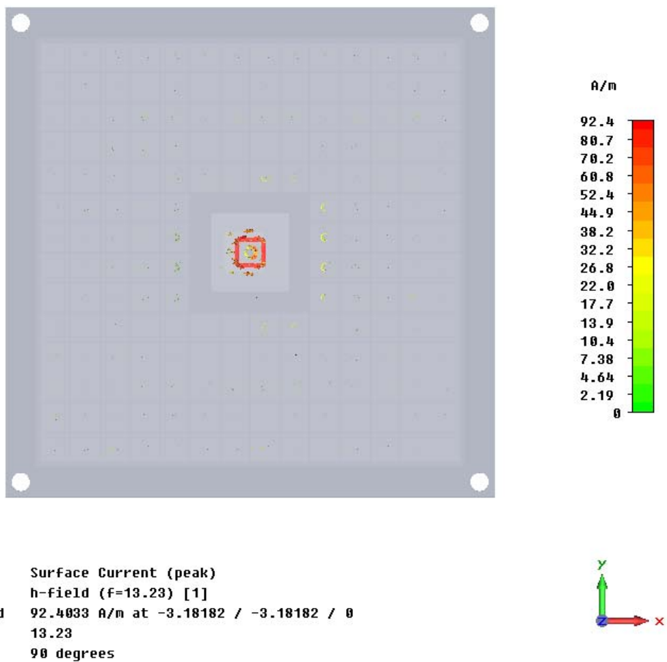
Fig. 5.7 – Surface current at 13.23 GHz, yellow circles surrounding the patch.
