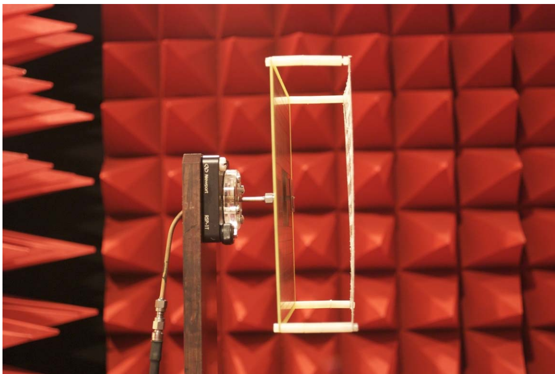
Fig. 6.10 – Fabry-Pérot suspended U-slot antenna mounted in the anechoic chamber
