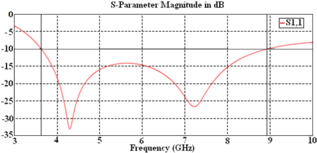
Fig. 4.5 – Return loss for the improved circular monopole antenna.
