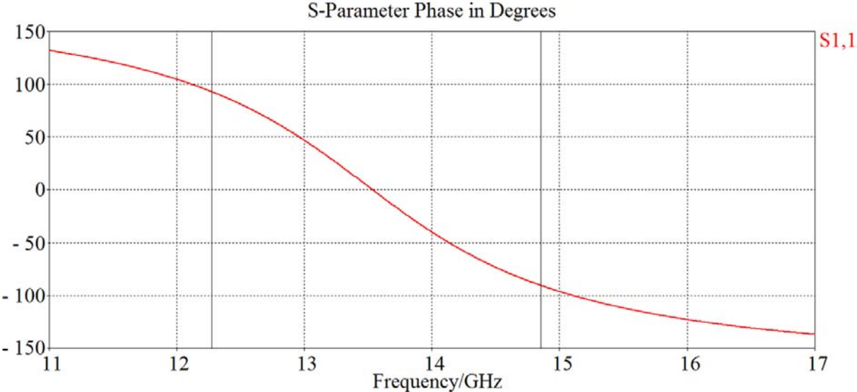
Fig. 5.5 – Reflection coefficient for the mushroom type HIS.
