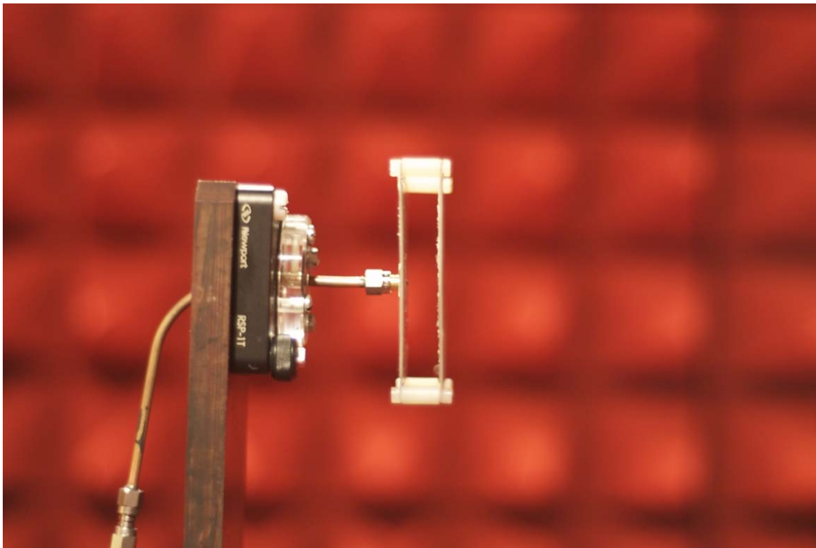
Fig. 6.7 – Fabry-Pérot patch antenna mounted in the anechoic chamber.
