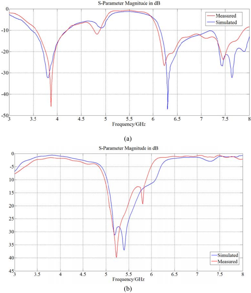
Fig. 4.26 – S11 (a) and S21 (b) parameters for the metamaterial-based stop band filter with three CSRRs etched do the ground plane: blue simulated and red measured.
