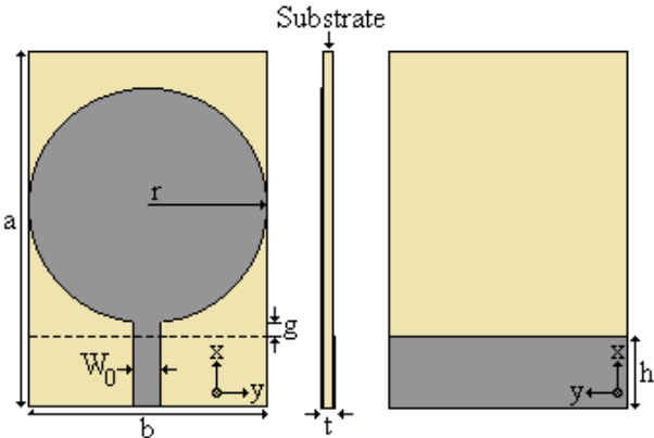
Fig. 4.2 – Circular monopole antenna, the gray region denotes a conductor material.
