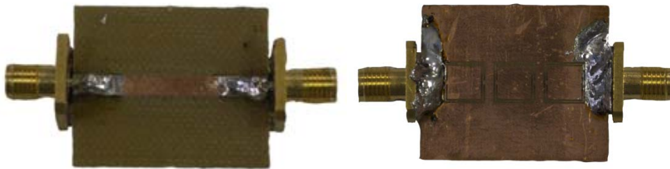
Fig. 4.25 – CSRR based filter prototype.
