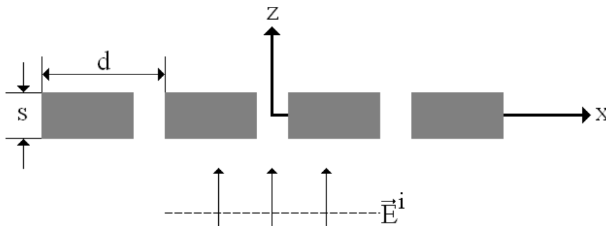
Fig. 3.3 – Metal screen illuminated by a normally incident plane wave [1].
