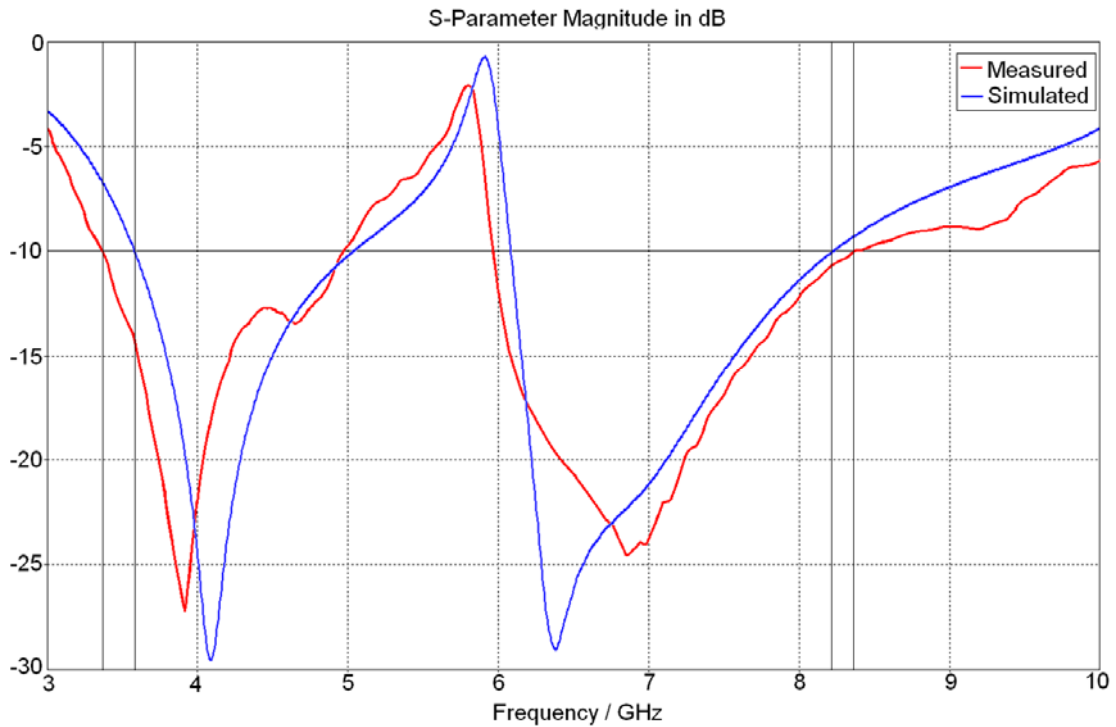
Fig 4.12 – Return loss for the circular monopole antenna, red measured and blue simulated results.
