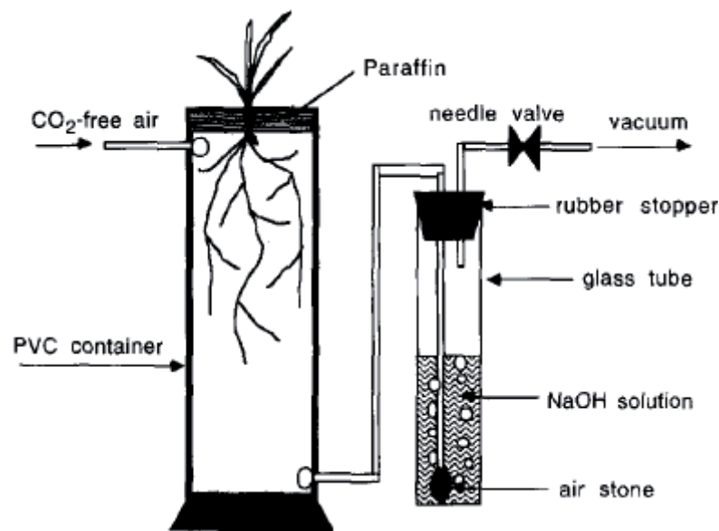
Figure 1.6. The method used to trap soil CO_2 efflux in alkali excluding the trapping of CO_2 from aboveground plant parts. (Cheng 1996).
