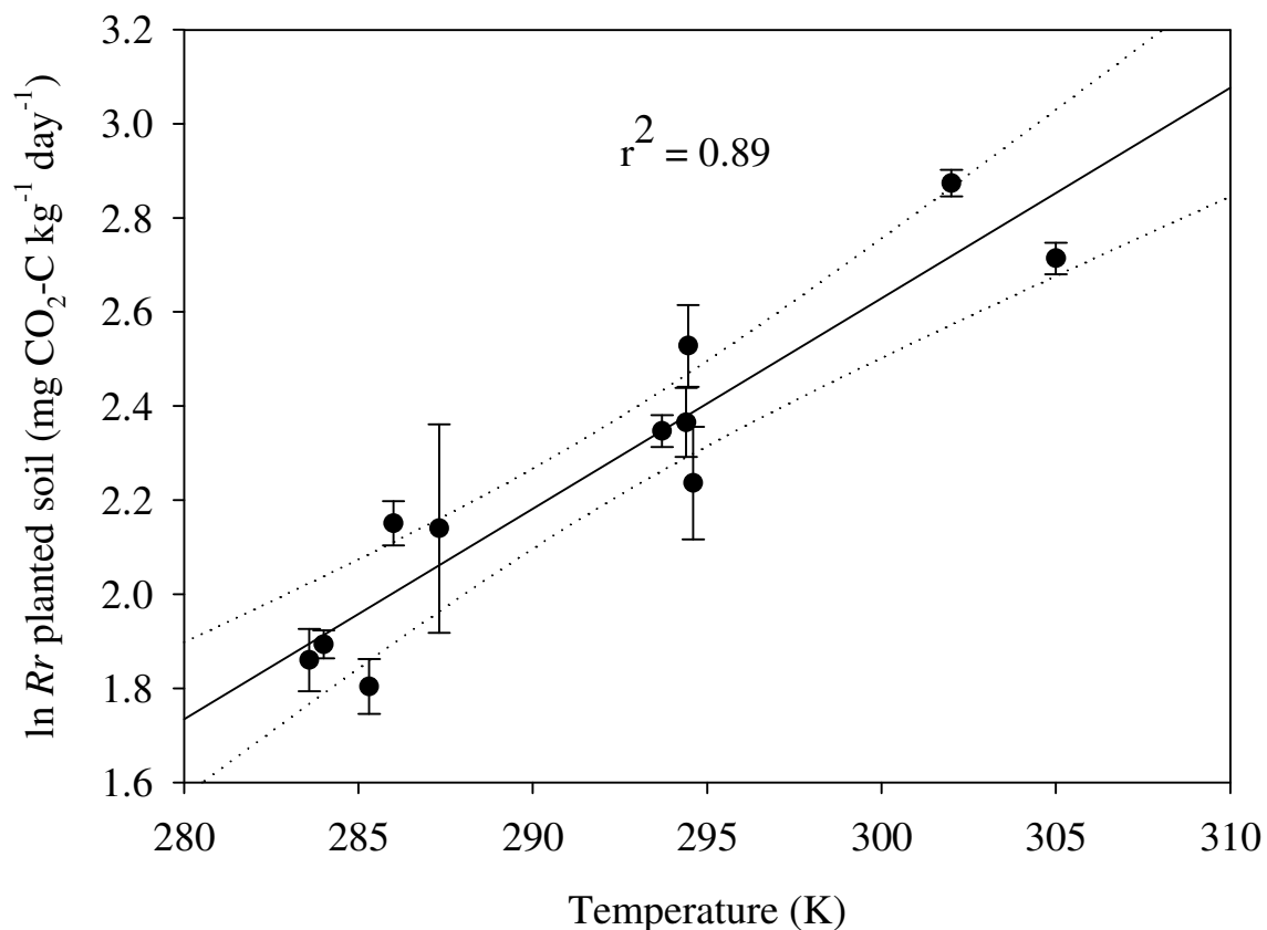
Figure 6. The response of recalcitrant soil C mineralization Rr ( \text{mg CO}_2\text{-C kg}^{-1} \text{ soil day}^{-1} ) in planted soils ( Lolium perenne ) to seasonal temperature variation when fresh C flux is not taken into account.
