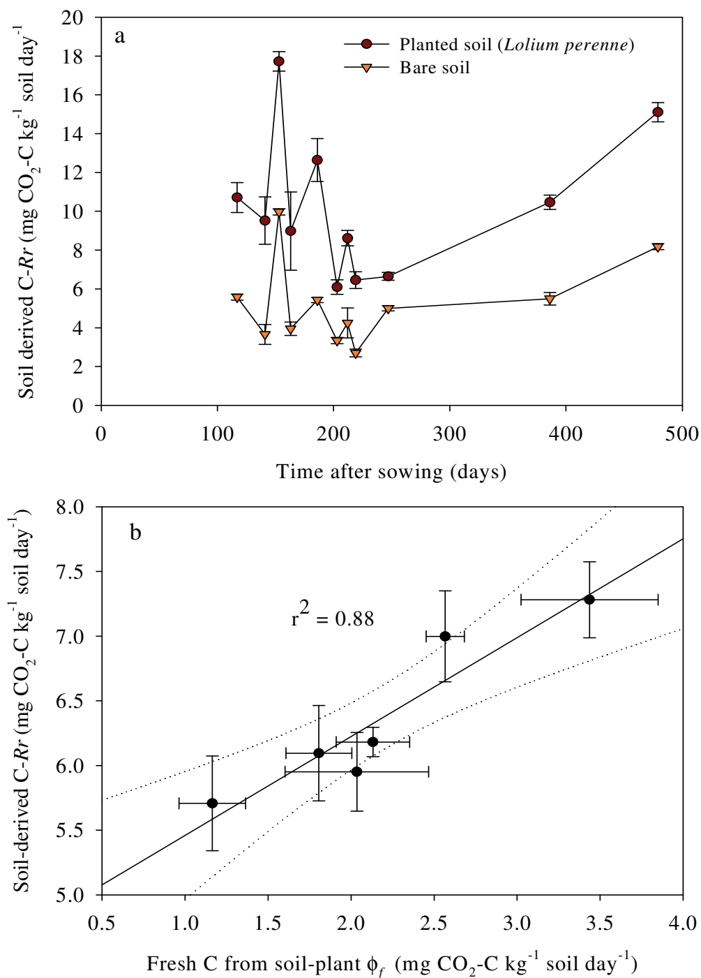
Figure 3. (a) Recalcitrant soil C mineralization (mg CO 2 -C kg -1 soil day -1 ) in control and planted ( Lolium perenne ) soils (b) relationship between fresh C and recalcitrant soil C mineralizations (mg CO 2 -C kg -1 soil day -1 ) in soil-plant system at mean daily temperature of 285 °C.
