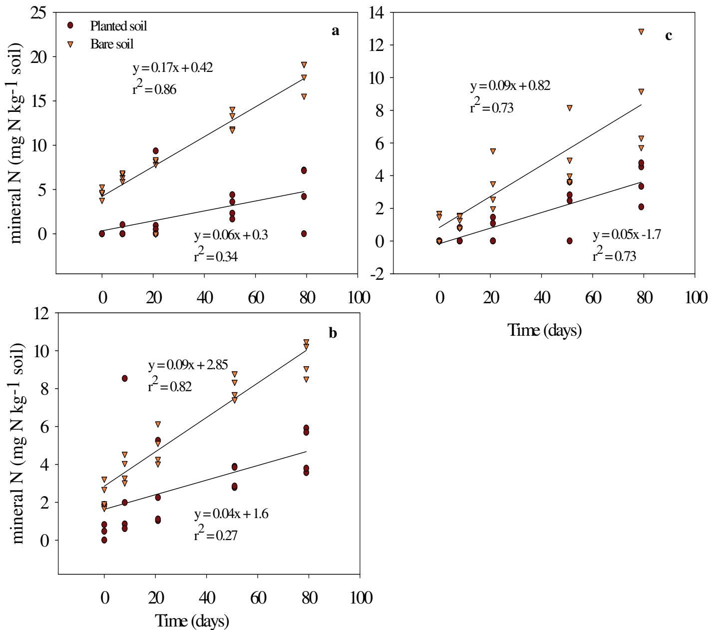
Figure 3: Net nitrogen mineralization in soils of upper (a) middle (b) and deep (c) horizons of planted and bare soils for 79 days of incubation.
