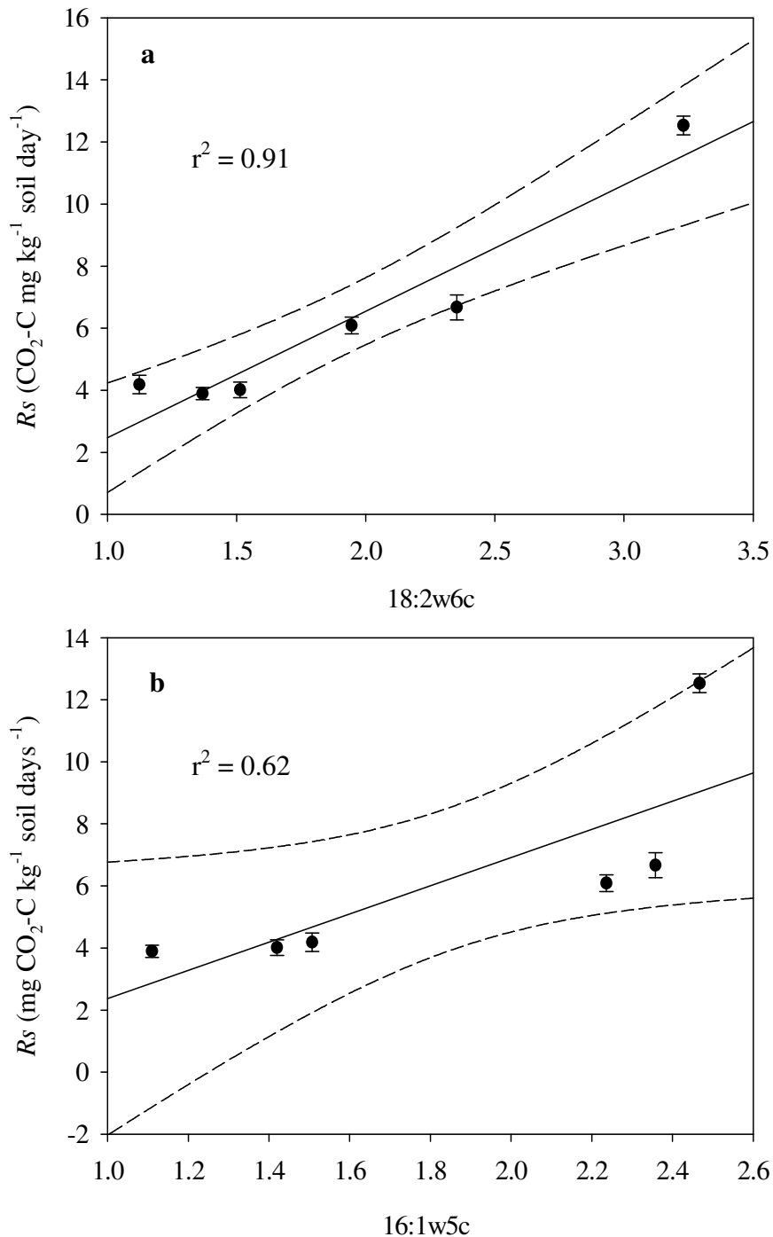
Figure 4: Correlation of saprophytic fungal biomarker 18:2 \omega 6c (a) and arbuscular mycorrhizae 16:1 \omega 5c with SOM mineralization i.e. soil-derived CO 2 -C. ( p -value <0.001, CI 95%).
