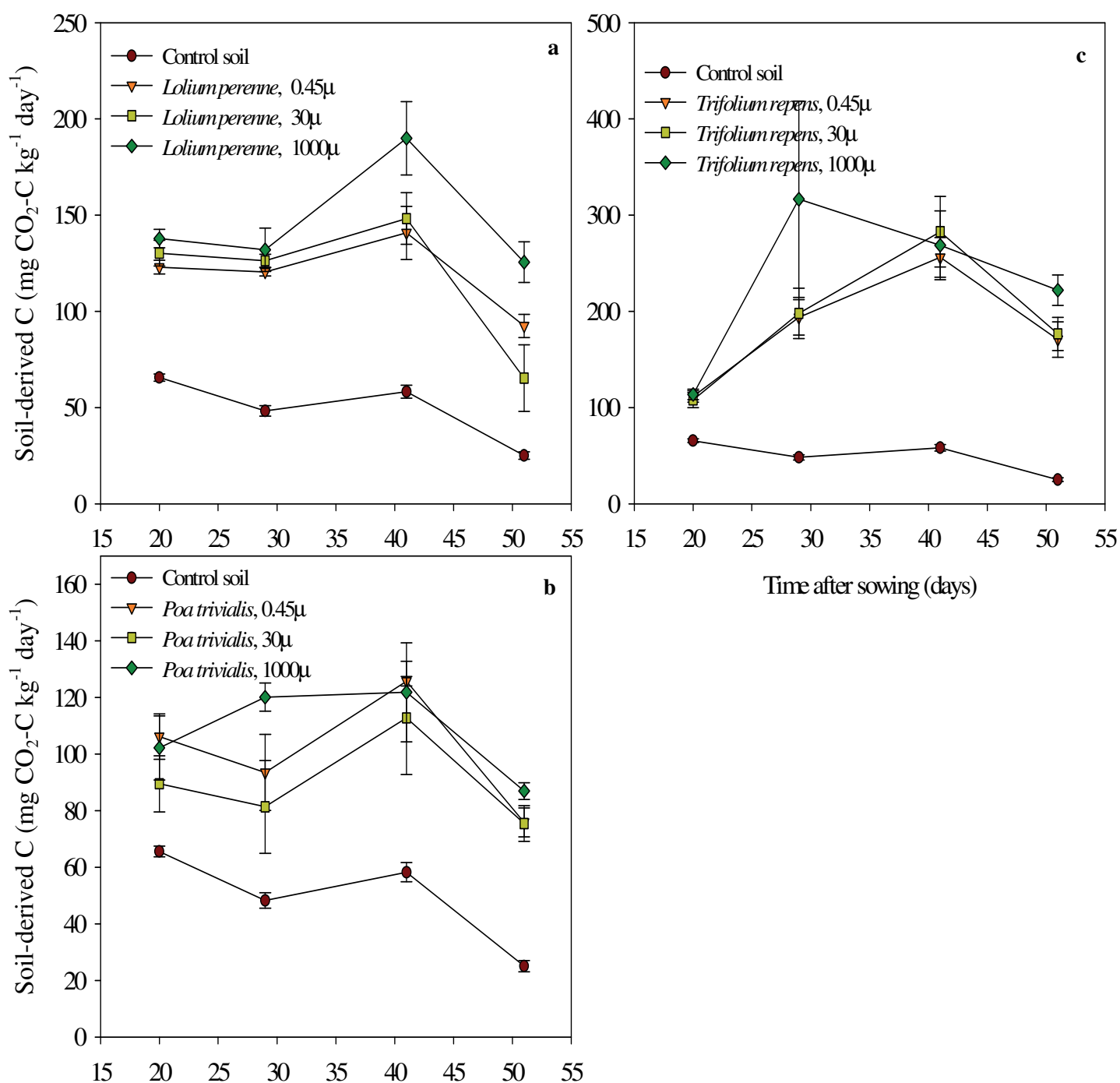
Figure 5.6. Soil derived C ( \text{mg CO}_2\text{-C kg}^{-1} \text{ soil day}^{-1} ) from control and Lolium perenne (a) Poa trivialis (b) and Trifolium repens (c) planted soils. 0.45 \mu , 30 \mu and 1000 \mu represent the soil compartments where only root exudates, root exudates and mycorrhizae and root exudates, mycorrhizae and roots have excess respectively.
