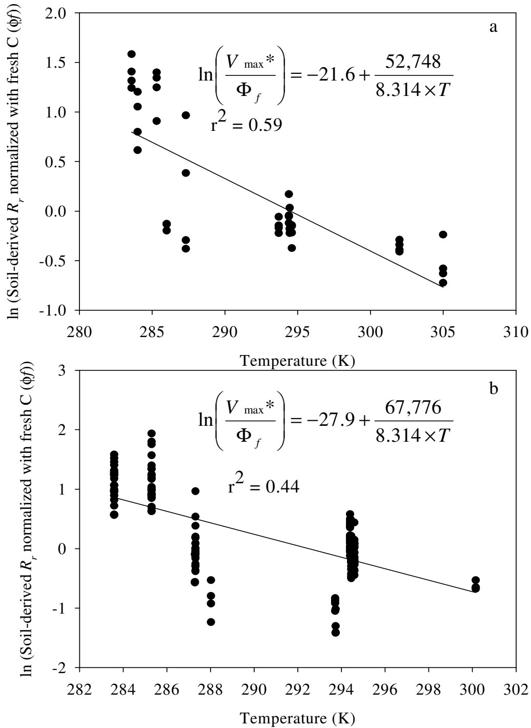
Figure 7. Experimental validation of the theory predicting negative effect of temperature (K) on recalcitrant soil C mineralization in steady-state system ( V_{\max}^* ). Results show that the mineralization of recalcitrant soil C decrease with warming in the plant-soil systems of (a) the model species Lolium perenne and (b) six other grassland species used to generalize findings, i.e. Trisetum flavescens , Poa trivialis , Festuca arundinacea , Bromus erectus , Brachypodium pinnatum and Trifolium repens . The rate of recalcitrant C mineralization is normalized with the flux of fresh C ( \Phi_f ) and adjusted with linearized form of Eq. 9 i.e.
