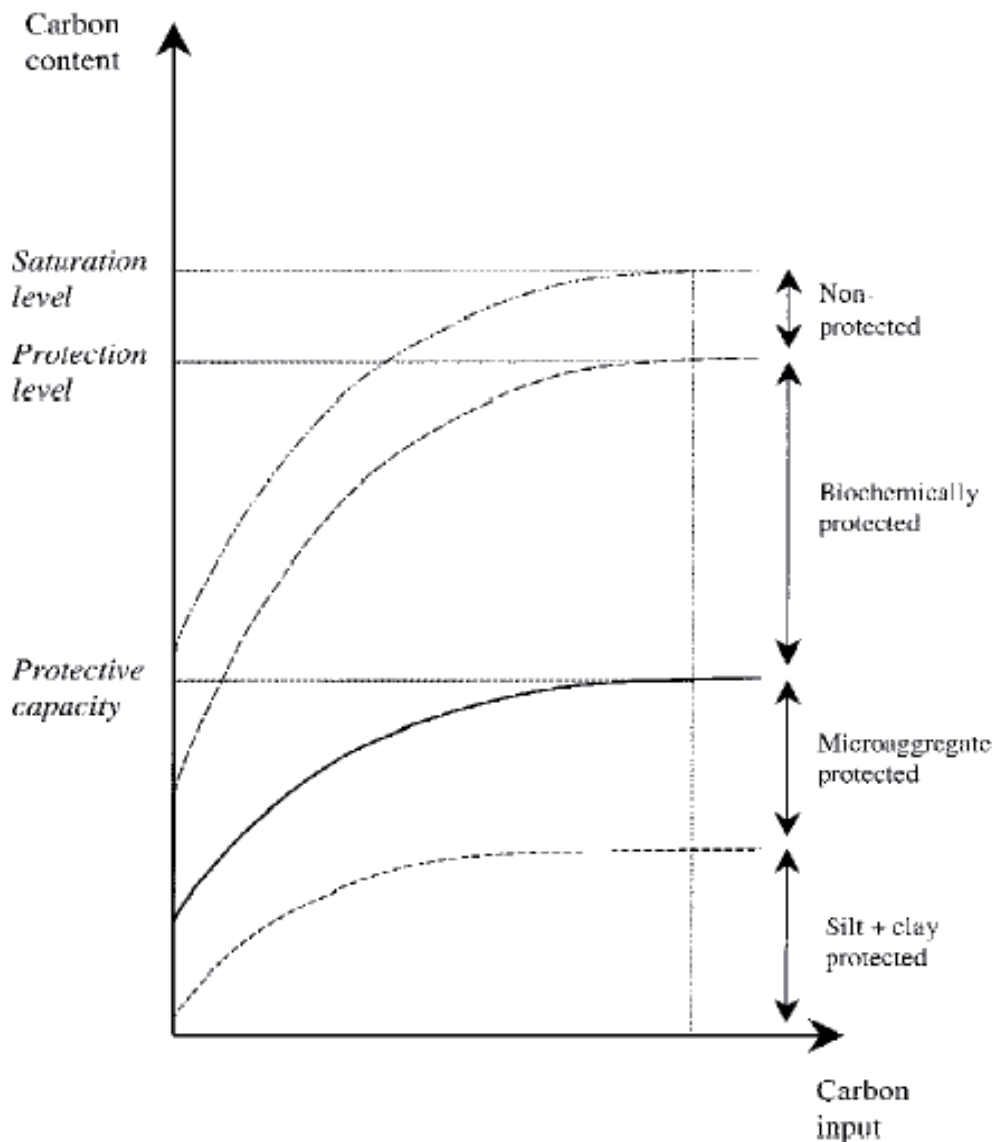
Figure 1.4. The protective capacity of soil (which governs the silt and clay and micro-aggregate protected C pools), the biochemically stabilized C pool and unprotected C pool define a maximum C content for soils. The pool size of each fraction is determined by their unique stabilizing mechanisms. (Six et al. , 2002)
