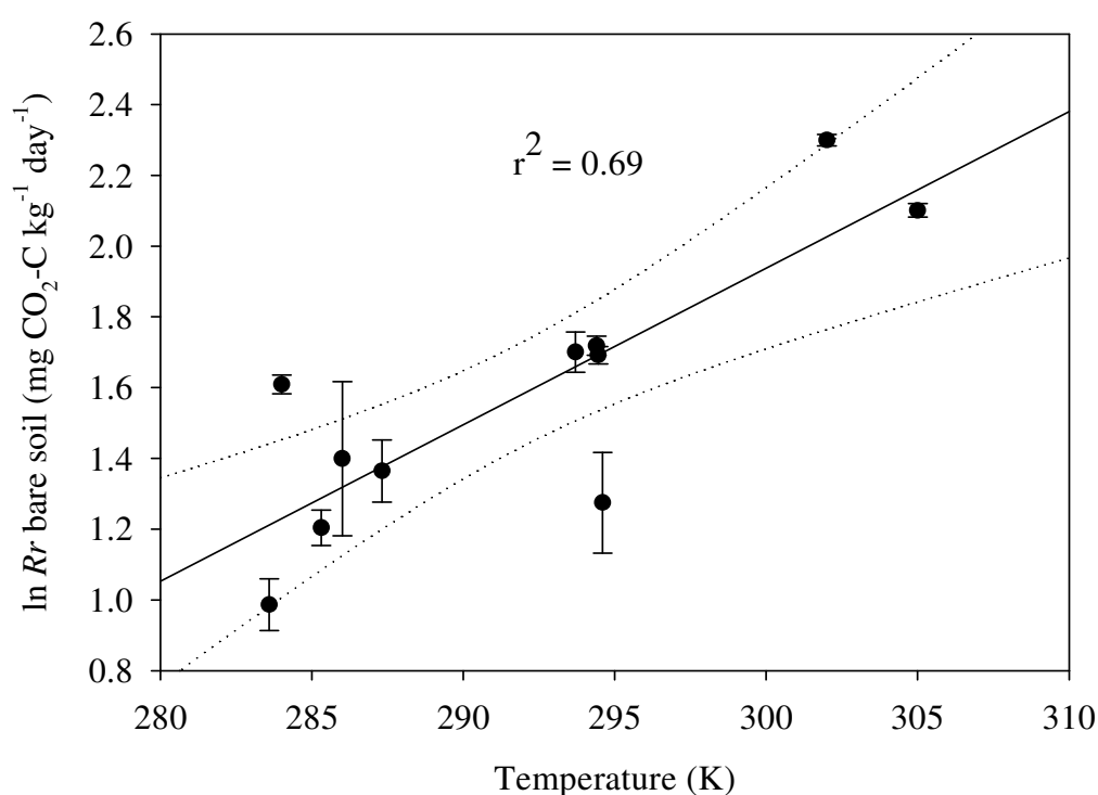
Figure 5. The response of recalcitrant soil C mineralization ( \text{mg CO}_2\text{-C kg}^{-1} \text{ soil day}^{-1} ) in bare soils to seasonal temperature.
