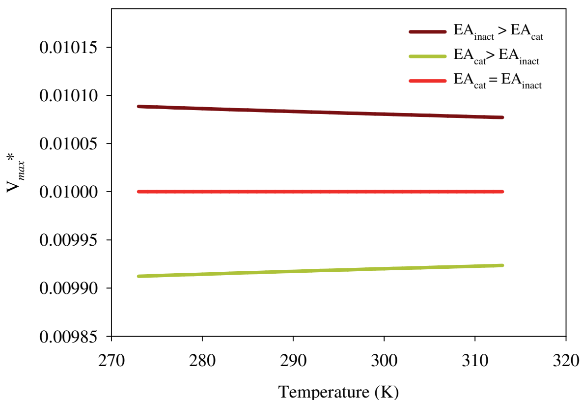
Figure 2. Effect of temperature on the velocity of an enzymatic reaction in a steady-state system as predicted by Eq. 9. Depending on values of EA_{\text{inact}} and EA_{\text{cat}} the temperature response of enzymatic reaction ( V_{max}^* ) can be positive, negative or null.
