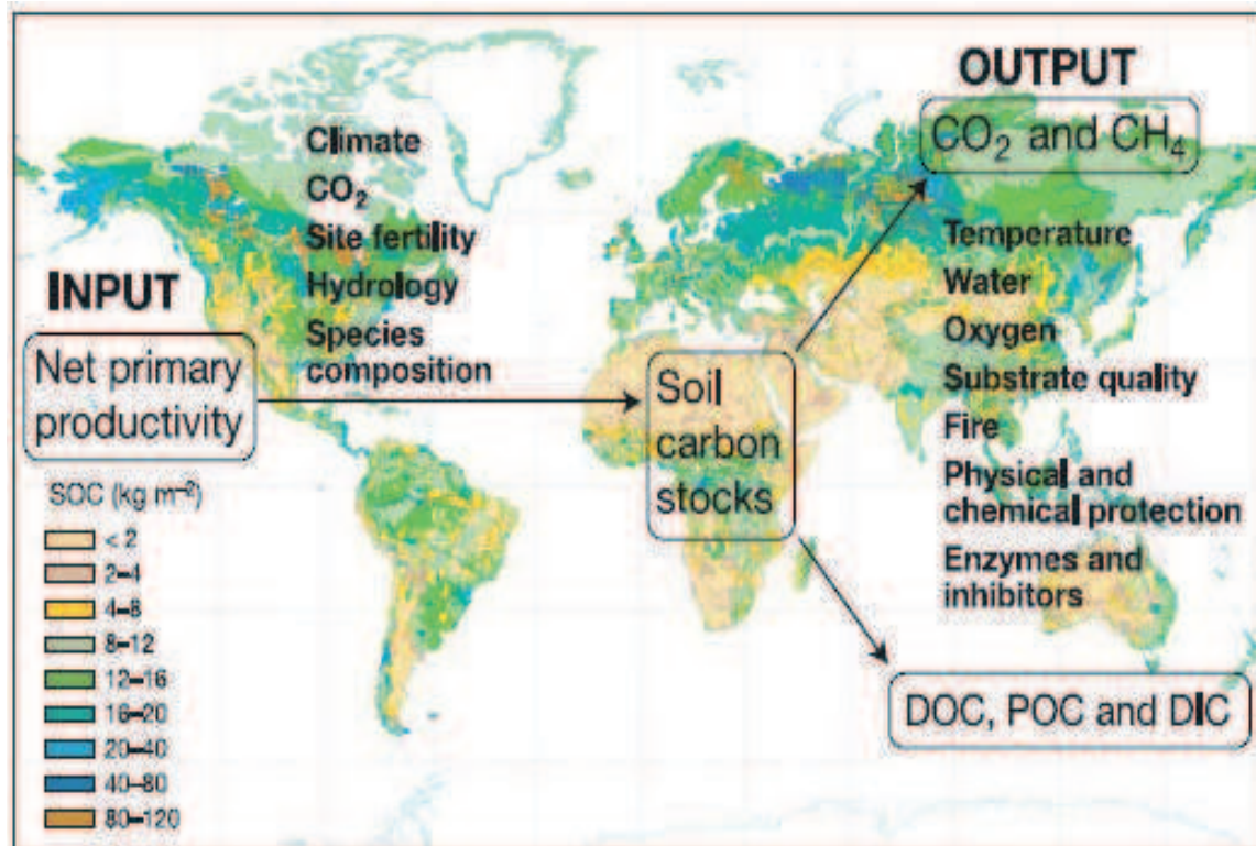
Figure 1.2. Factors controlling the main inputs and outputs of soil C, superimposed over a global map of soil organic C stocks (Miller projection; 1 : 100,000,000 for background map). Taken from Davidson & Janssens (2006).
