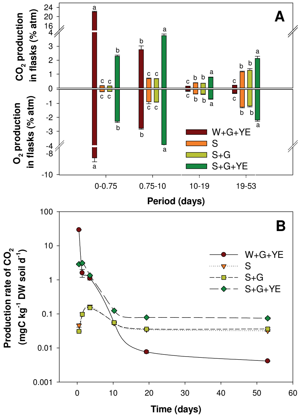
Figure 3: Acellular respiration induced by cell-free yeast extract incubated in water and soil microcosms
