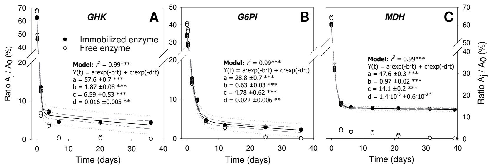
Figure 4: Enzymatic activities in the soil of Theix.
