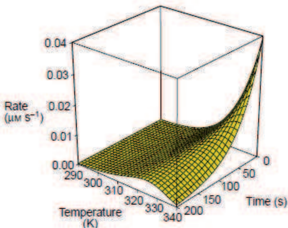
Figure 1. Temperature dependence of enzyme activity in an enzyme assay. The variation of enzyme activity with temperature (290-340 K) and time (0-200 s) during the assay was simulated using Eq 6 with following parameter values k_{cat} = 80 \text{ KJ mol}^{-1} , k_{inact} = 95 \text{ KJ mol}^{-1} , total enzyme concentration = 100 nM.
