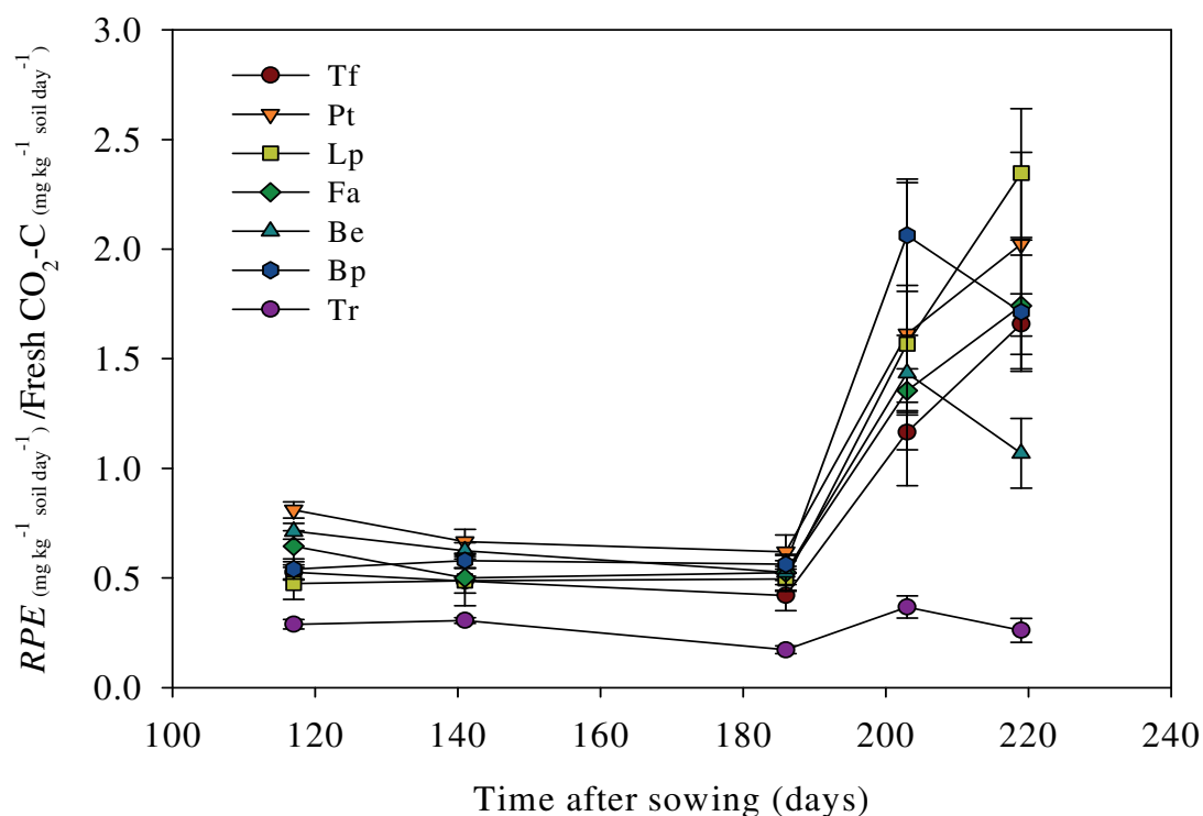
Figure 5.2. Rhizosphere priming effect ( \text{mg CO}_2\text{-C kg}^{-1} \text{ soil day}^{-1} ) expressed per unit of fresh C ( \text{mg CO}_2\text{-C kg}^{-1} \text{ soil day}^{-1} ) respired from soil-plant system.
