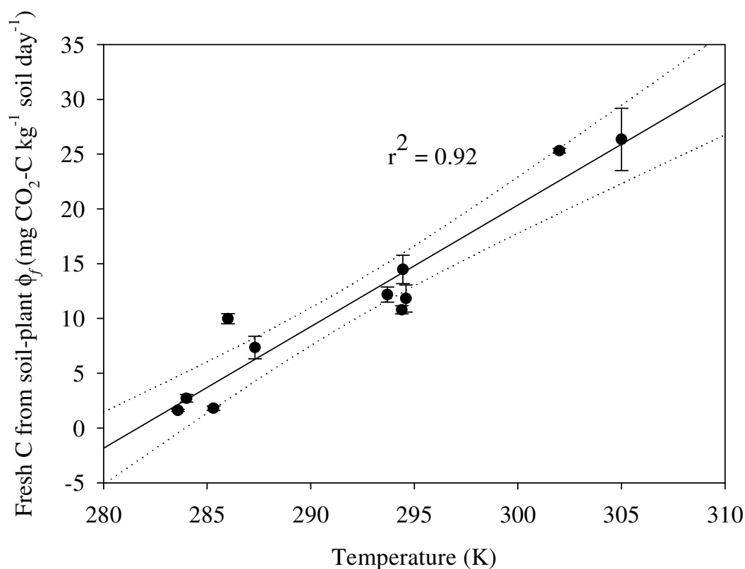
Figure 4. Effect of seasonal temperature (K) on the respiration of fresh C on the respiration of fresh C ( 13 C-labelled) flux (mg CO 2 -C kg -1 soil day -1 ) from soil-plant system of Lolium perenne .
