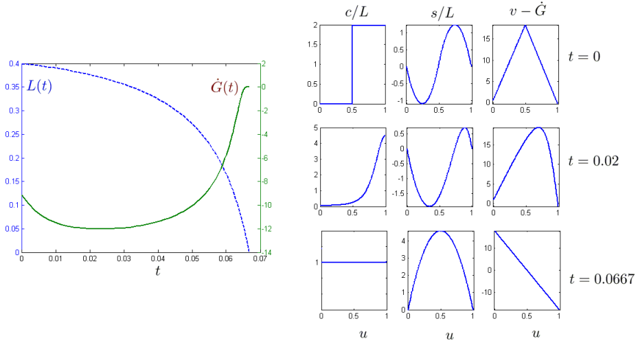
Figure 3.19: L(t) , \dot{G}(t) and profiles c/L , s/L = \mathcal{K}^{\frac{\sigma+(L-1)}{L}} and v - \dot{G}(t) for parameters \mathcal{P} = 0.245 , \mathcal{K} = 150 (See Fig.3.12) and c_0 = 1 . Starting from the L_i = 0.4 and a concentration fully biased to the front.
