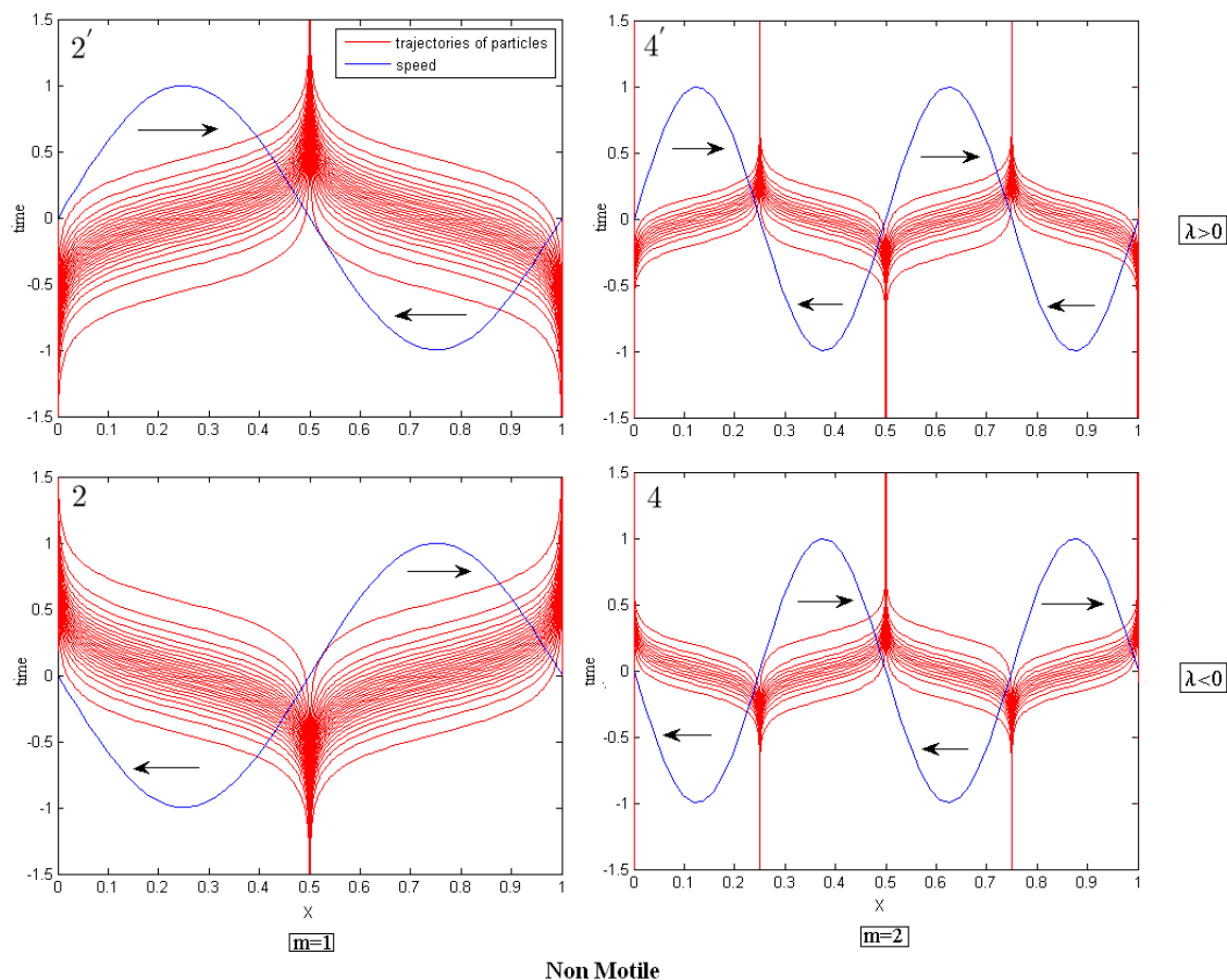
Figure 3.26: Trajectories of particles from sources to sinks for the first two non motile bifurcation points for initially homogeneously distributed set of particles . Labels 2, 2', 4, 4' are related to Fig.3.12 and Fig.3.13.
