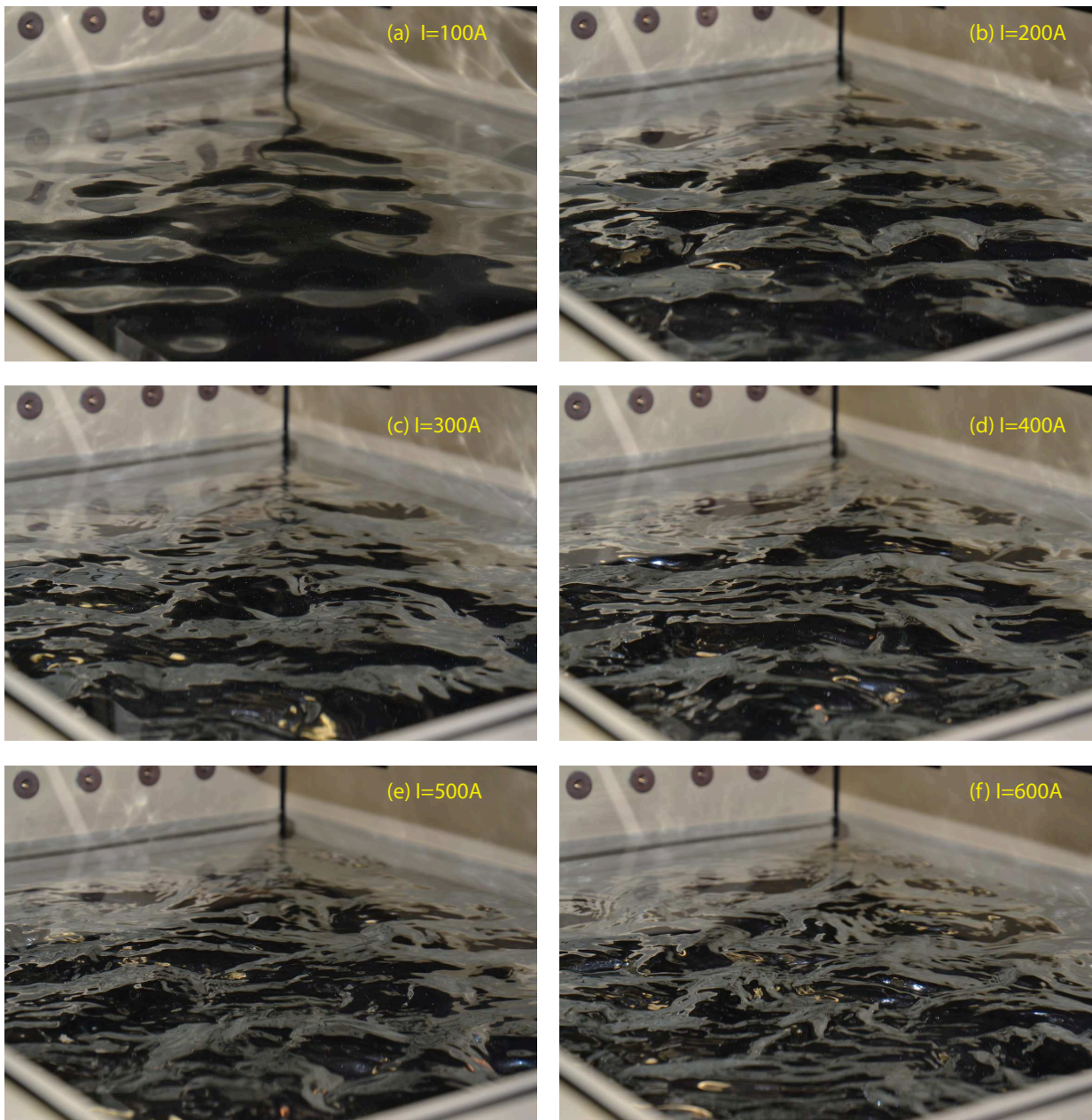
Figure 5.1: Photos of the experiment for increasing forcing strength, Regular forcing.
