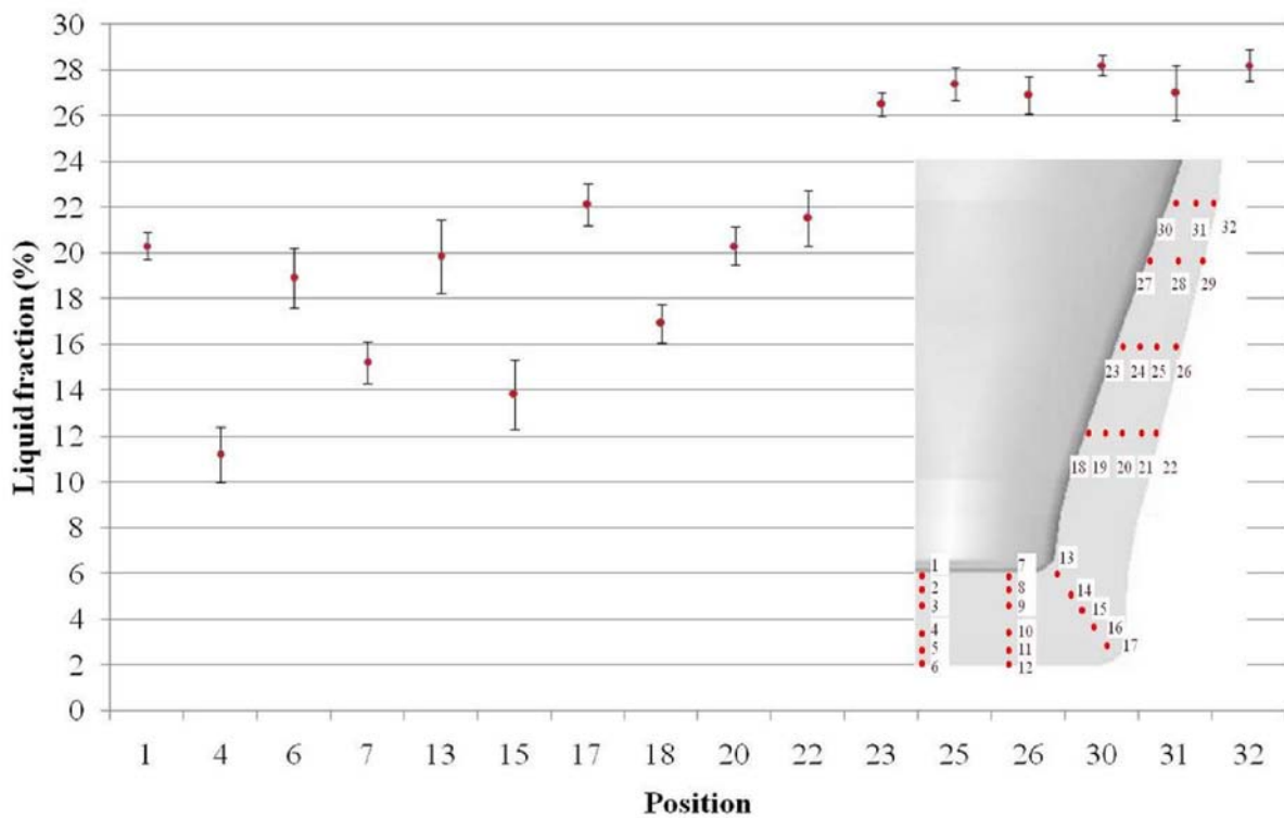
Fig. 4.25. Liquid fraction vs position of the thixoforged part (T billet = 1320^{\circ}\text{C} ).
