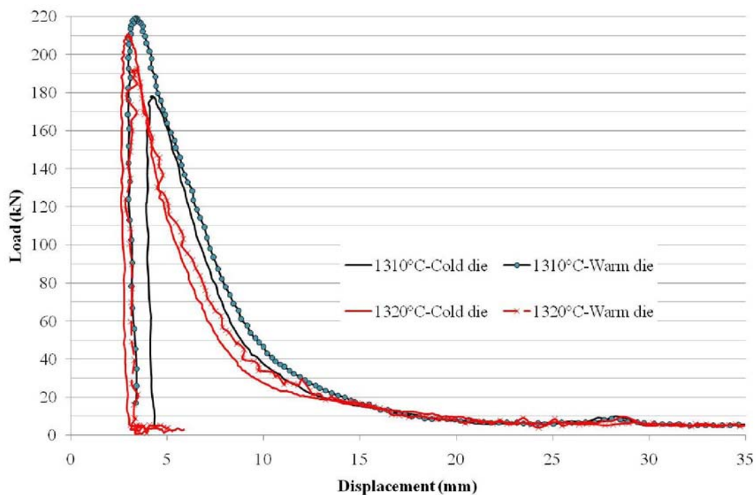
Fig. 4.17. Load-displacement curves of the thixoforging process at the same billet temperature but with various die temperatures.
