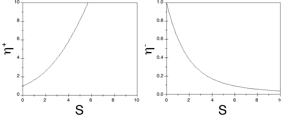
Figure 3.10.: Variation of the auxiliary parameters \eta_- and \eta_+ with phase-mismatch.
