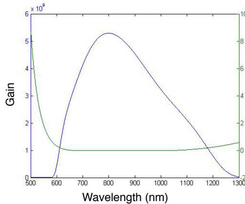
Figure 2.5.: (blue) Gain in function of the wavelength for a pump at 400\text{nm} and a seed centered at 800\text{nm} , (green) spectral phase accumulated due to OPA for each wavelength.
