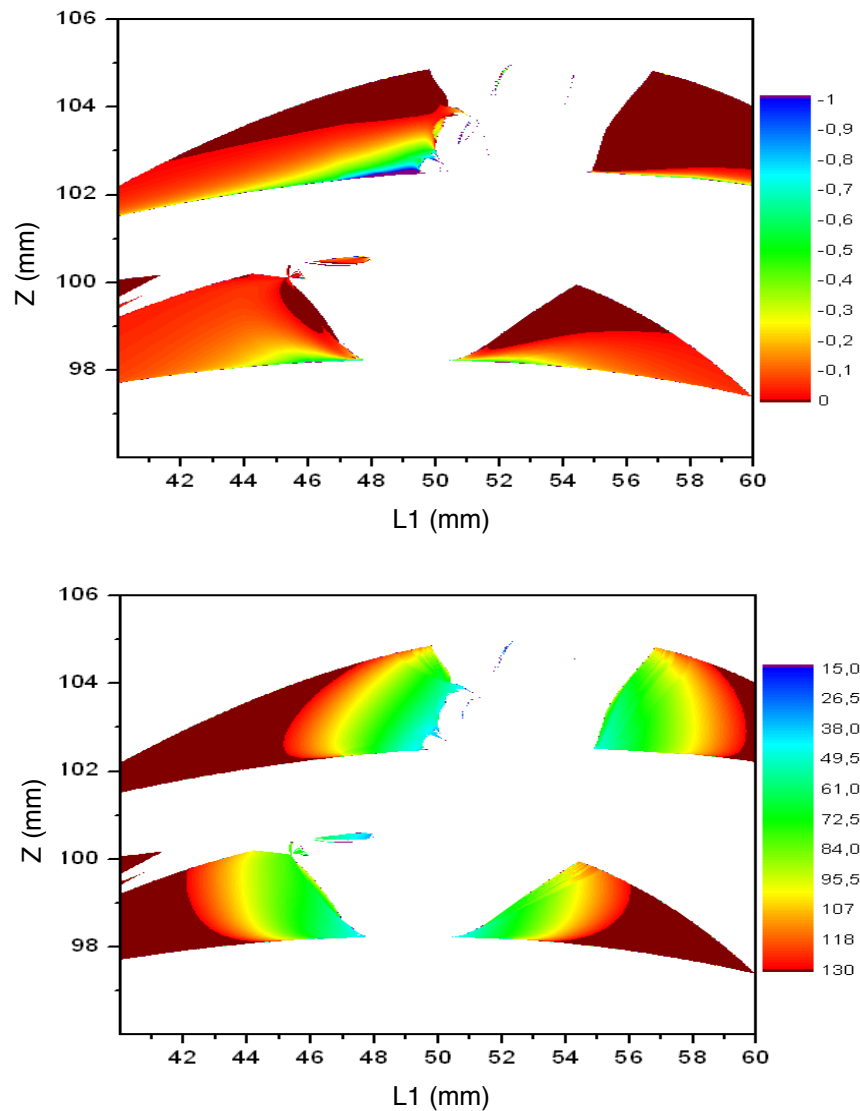
Figure 2.20.: (Bottom) ML beam size (in \mu\text{m} ) as a function of the sub-cavity dimensions (in \text{mm} ); (Top) the ML parameter.
