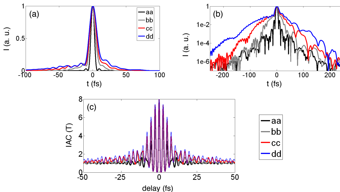
Figure 4.5.: Pulses with fourth order chirp. aa to dd represent pulses with 5.98 fs, 9.46 fs, 11.28 fs, 13.40 fs, fourth order chirp values of 0 \text{ fs}^4 , 1800 \text{ fs}^4 , 3600 \text{ fs}^4 , 5400 \text{ fs}^4 . Intensity profile on (a) a linear and (b) a logarithmic scale. (c) The corresponding IAC traces.
