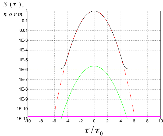
Figure 3.18.: TOCC profile in logarithmic scale for a noise level of n = 1e^{-6} , \frac{T}{\tau_0} = 10^7 , considering that \tau_0 = 10 fs, T = 0.1 \mu\text{s} .
