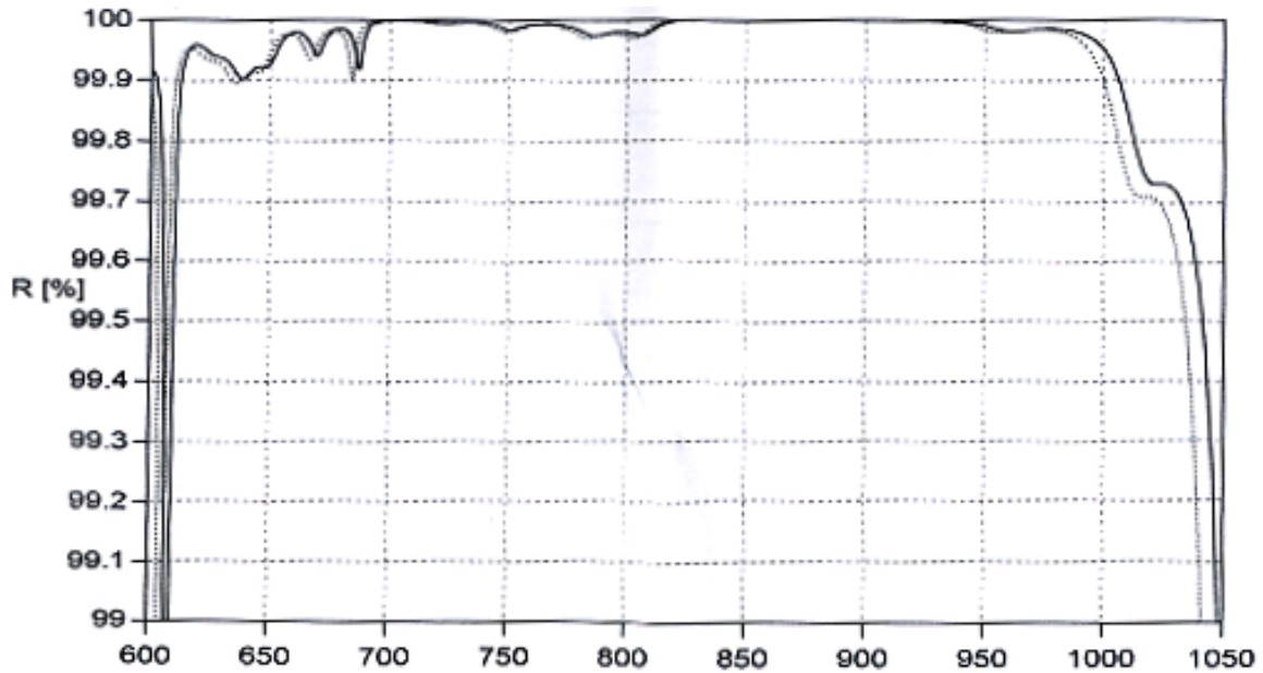
Figure B.7.: Reflective coefficient for the back-end mirror M4 (G0304008). The continuous line is at 0^\circ incidence and the traced line for 10^\circ incident angle.
