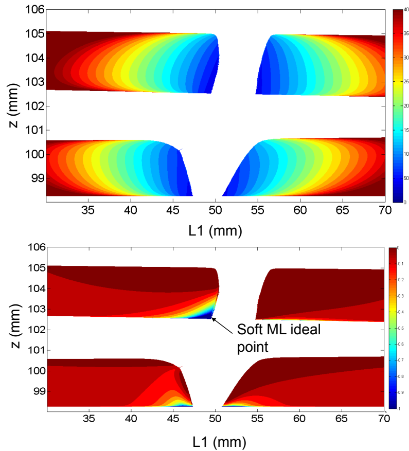
Figure 2.13.: (Top) ML beam size (in \mu\text{m} ) as a function of the cavity dimensions (in \text{mm} ); (Bottom) the ML parameter as given by Eq. (2.34). The soft aperture ML position is indicated.
