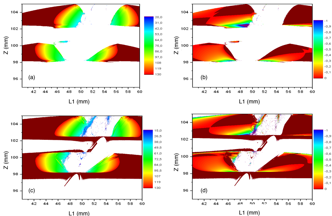
Figure 2.25.: ML using an adaptable pump size. (a) ML spot size ( \mu\text{m} ) and (b) ML parameter as calculated by the algorithm in Fig. (2.9); (c) ML spot size ( \mu\text{m} ) and (d) ML parameter as calculated by the algorithm in Fig. (2.14).
