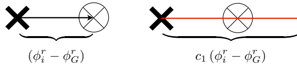
Figure 4.42.: 1D PSO. A particle position represented by the black cross and an attractor represented by the reticule. The red line represents the possible positions the particle can take in the next interaction due to the attractor.
