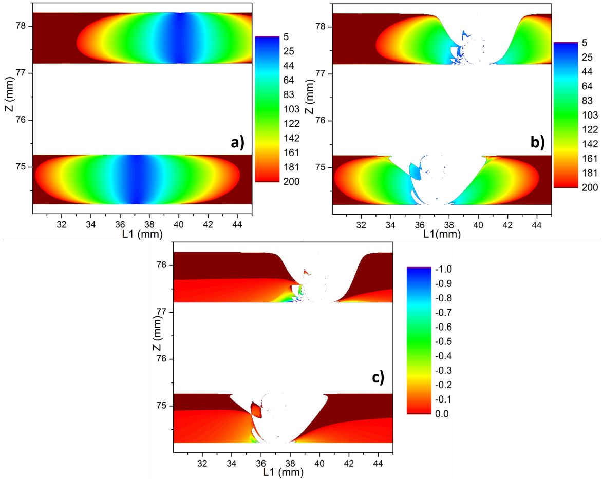
Figure 2.32.: a) CW beam size ( \mu\text{m} ), b) ML beam size ( \mu\text{m} ), c) ML parameter as given by Eq. (2.34). ML results obtained using the algorithm of Fig. (2.9).
