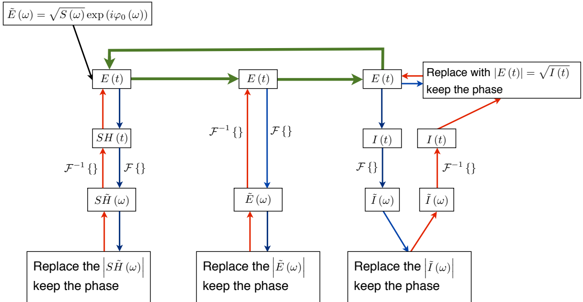
Figure 4.24.: Alternative Gerchberg-Saxton algorithm for spectral phase retrieval. Subroutines are given by the blue/red arrows. The green arrows explicit the behavior of the main routine.
