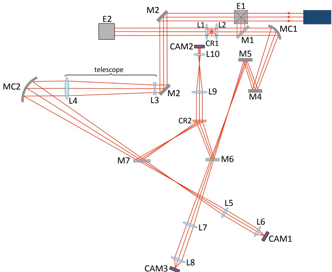
Figure 5.19.: Single shot cross-correlator based on a sagittal astigmatic line. M1-7 are plane mirrors, L1 and L2 are two cylindrical 0.35 NA lenses. L5-L10 are pairs of imaging 2f_1 - 2f_2 systems, L3-L4 is a telescope; E1 is a crossed elevator (descendent); E2 is an elevator (ascendent); MC1 and MC2 are curved mirrors. CR1 is the second harmonic crystal and CR2 the SFG crystal wedge crystal.
