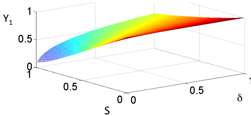
Figure 1.4.: Maximum conversion of the idler square amplitude given by the parameter \gamma_1 as a function of the phase mismatch parameter S and the intensity ratio parameter \delta .
