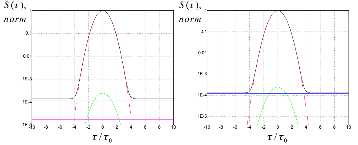
Figure 3.17.: TOCC profile in logarithmic scale for a noise level of n = 1e^{-4} , (right) \frac{T}{\tau_0} = 10^7 , considering \tau_0 = 10 fs, T = 0.1 \mu\text{s} and (left) \frac{T}{\tau_0} = 10^5 considering \tau_0 = 10 fs, T = 1 ns.
