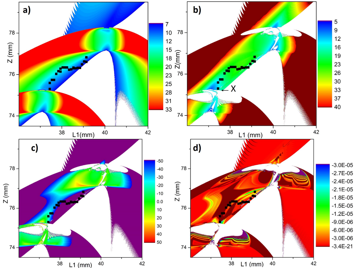
Figure 2.33.: Results of the algorithm that adapts the pump size to the spot size. (a) pump spot size, in \mu m ; (b) the CW mode spot size, in \mu m ; (c) the difference between the two using \delta w , in percentage (zero means there is no difference); (d) the ML parameter as given by Eq. (2.33) in W^{-1} . Experimental points are shown in black; the "X" refers to the point where the largest spectrum was found.
