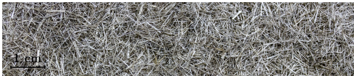
FIGURE 5.2 – Fibres de lin FRD ® Fibras-S ® 6A
