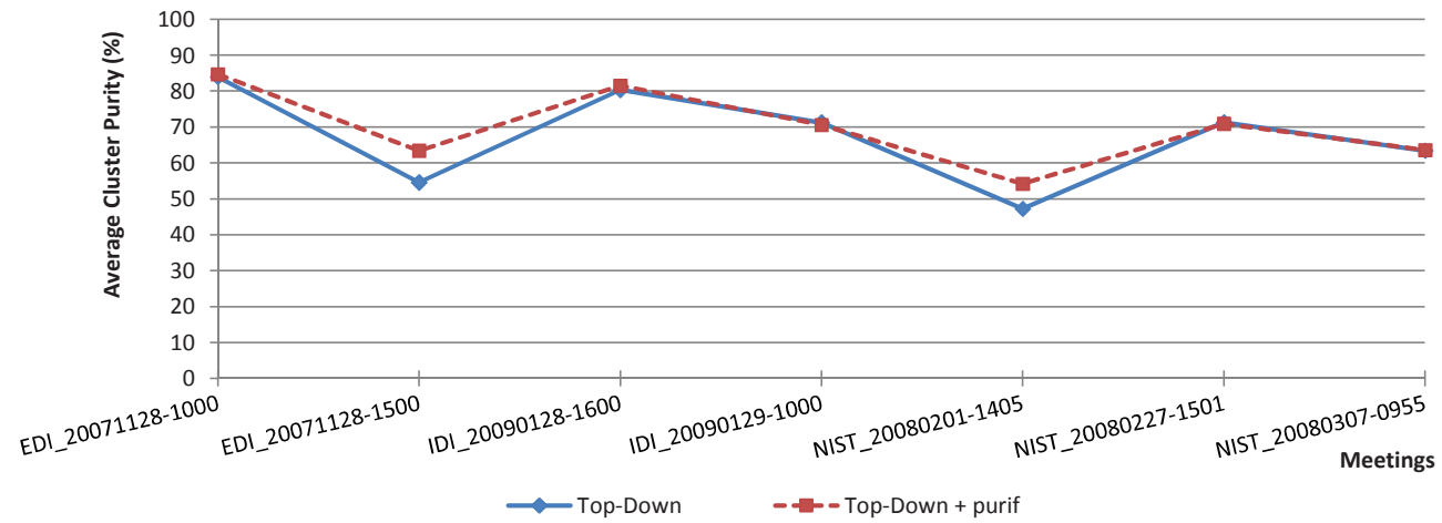
(b) NIST RT'09 dataset (SDM condition)
