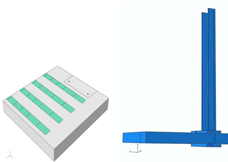
FIGURE 6.3 – Les parties composant la dalle 3
