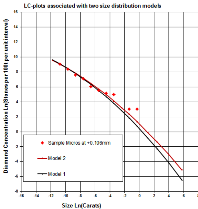
Figure 4-15 : LC-models for two size distribution models. Model 1 suggests a grade of 13cphat and model 2 a grade of 25cphat at +5diamond sieve bottom cut-off. The need for confirmation of the models by means of macrodiamond sampling is clear.
