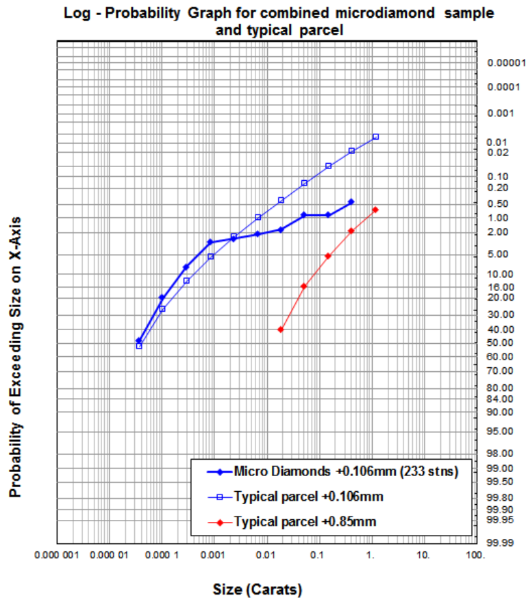
Figure 4-2 : Sample and Model Log-Probability graphs. Sampling data is shown at bottom truncation of 0.106mm.
