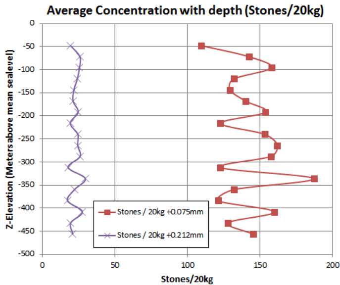
Figure 6-3 : Diamond concentration in 24m benches with depth
