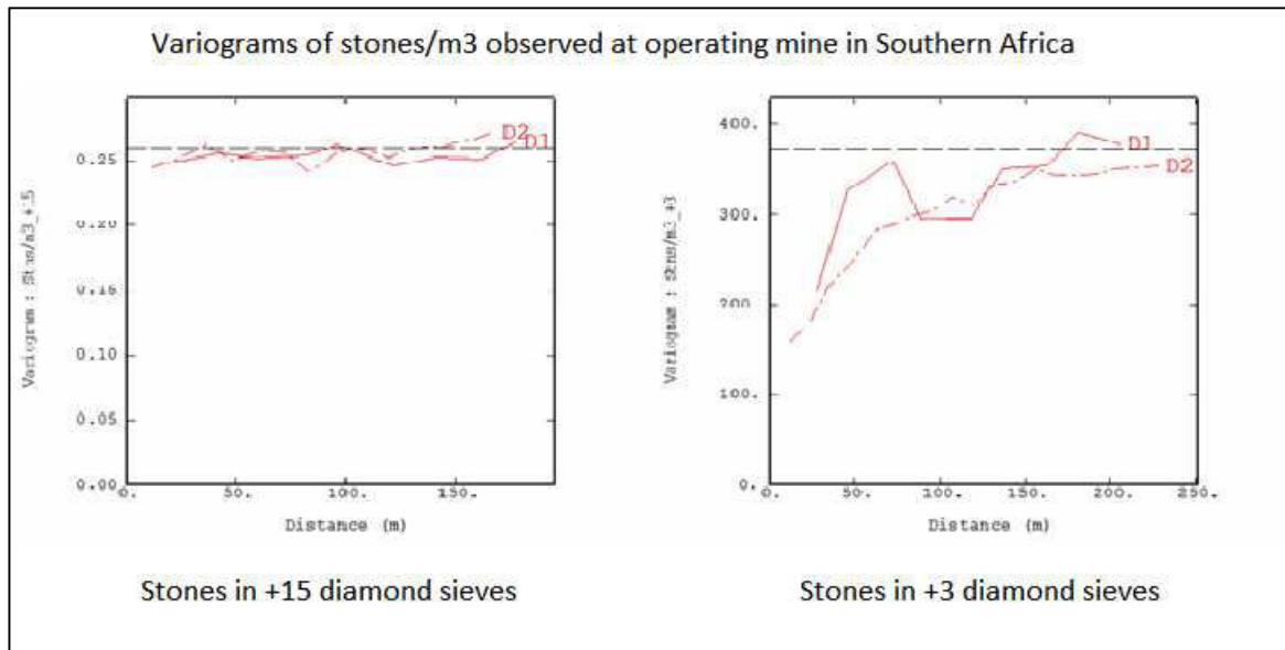
Figure 3-2 : Loss of spatial structure with increase in bottom truncation size
