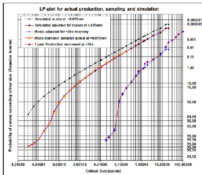
Figure 7-1 : Current mine LP-curve for production and sampling
