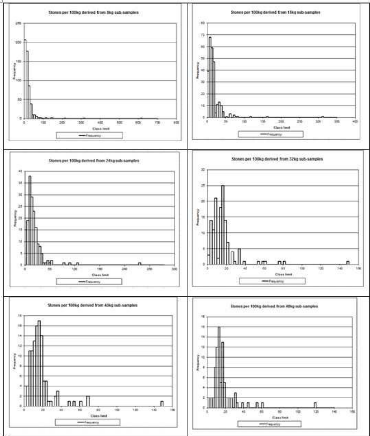
Figure 4-10 : Histograms of Sample concentrations per 100kg for all possible 8, 16, 24, 32, 40 and 48kg subsamples from Phase I and II sampling.
