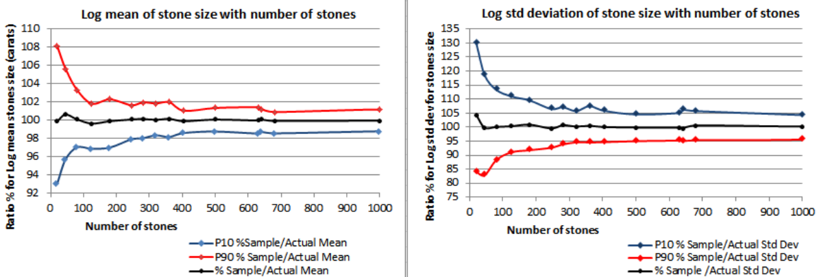
Figure 4-21 : Confidence bands for mean and standard deviation of stone size distribution
