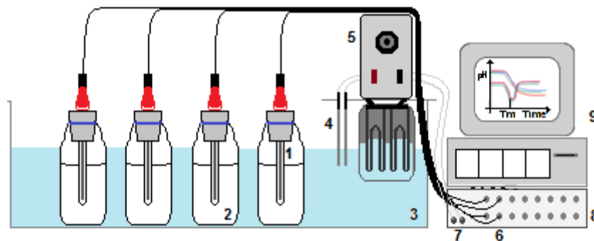
Fig. 1 Cinac System simplified diagram (adapted from Wang, 2005).
