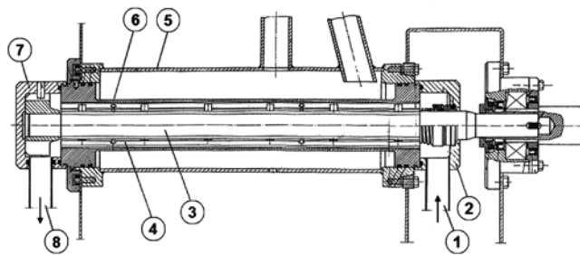
Fig. 5.2.1. Schematic representation of the SSHE WCB® Model MF 50. 1. Inlet connection for sorbet mix. 2. Inlet cover bowl. 3. Rotor. 4. Scraper blades rows. 5. Heat exchange cylinder jacket with vaporizing r22. 6. Heat exchange cylinder. 7. Outlet cover bowl. 8. Outlet pipe for sorbet.
