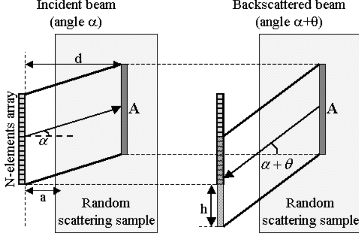
FIG. I.21: Effect of the array finite aperture on the single scattering intensity obtained after beamforming. On the left is depicted the area A sounded by an incident beam corresponding to a plane-wave with an incident angle \alpha , at a distance d(= a + ct/2) from the array. On the right, the backscattered beam at an angle \alpha + \theta comes from A and intercept then only a fraction of the array. h is the size of the beam scattered out of the array.
