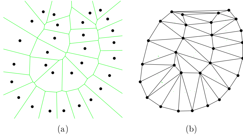
Figure 2.3: (a) Voronoi diagram of a set of points in the plane. (b) Its dual Delaunay triangulation.
