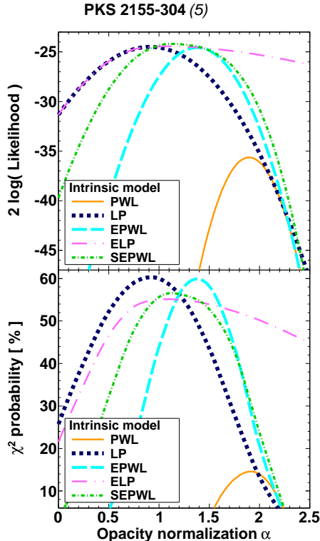
FIGURE 5. Top panel: Likelihood profiles, as a function of the optical depth normalization for the different intrinsic models which are detailed in the legend. Bottom panel: Corresponding \chi^2 probabilities as a function of the optical depth normalization. The SEPWL is the spectral model chosen to describe the spectrum of PKS 2155-304 (5).
