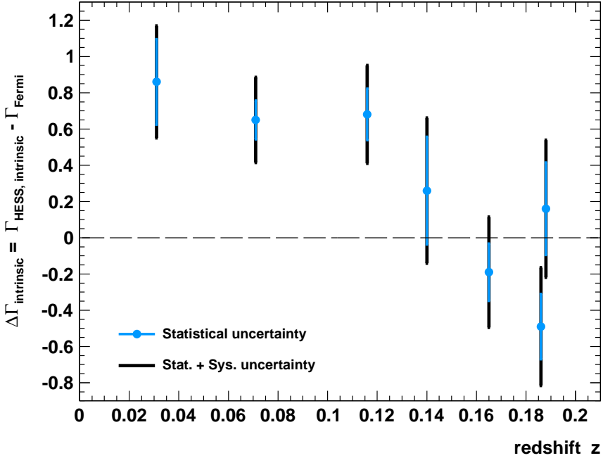
FIGURE 12. Preliminary intrinsic break measured with H.E.S.S. and Fermi -LAT after EBL de-absorption
