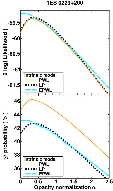
FIGURE 4. Top panel: Likelihood profiles, as a function of the optical depth normalization for the different intrinsic models which are detailed in the legend. Bottom panel: Corresponding \chi^2 probabilities as a function of the optical depth normalization. The PWL is the spectral model chosen to describe the spectrum of 1ES 0229+200.
