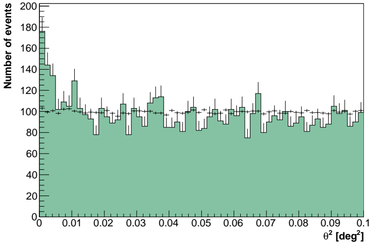
FIGURE 12. Distribution of the squared angular between the arrival direction of the \gamma rays and the direction of 1ES 1312-423. The filled histogram shows the ON events while the background derived from the OFF regions is shown with crosses.
