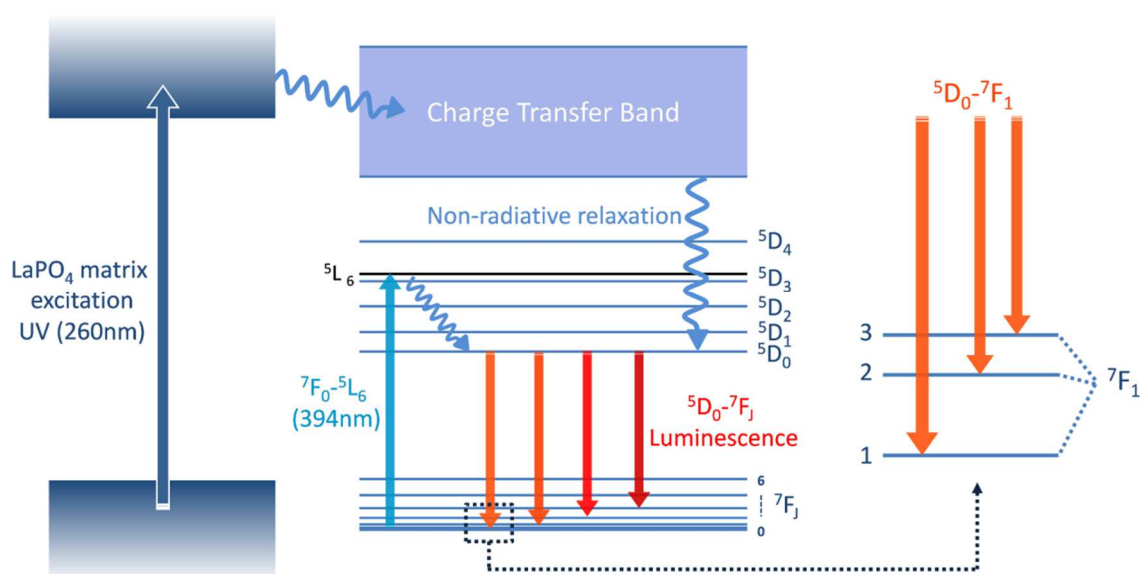
Figure 4.3. Energy level scheme of \text{LaPO}_4:\text{Eu} photoluminescence. The two main excitation pathways through the \text{LaPO}_4 matrix by UV (260nm) and the direct 7\text{F}_0-5\text{L}_6 excitation by 394nm, and the 5\text{D}_0-7\text{F}_J emission lines are noted. The right scheme zoomed from the dotted square shows the low symmetry splitting into the three sublevels of 7\text{F}_1 .
