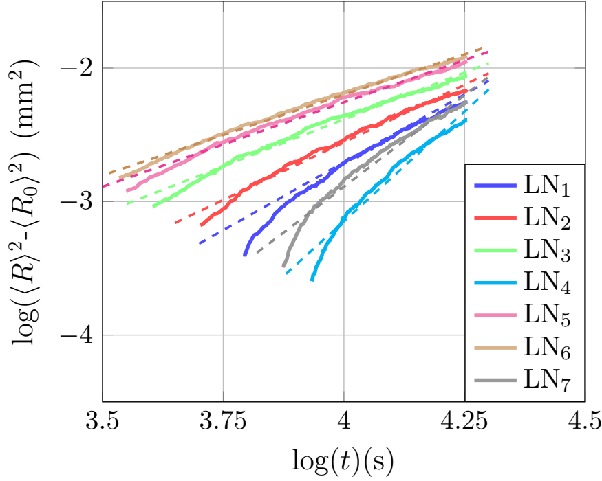
Fig. 2.14. Evolution of \log(\langle R \rangle^2 - \langle R_0 \rangle^2) as a function of \log(\text{time}) according to full field results. Linear approximations are added in dashed lines.
