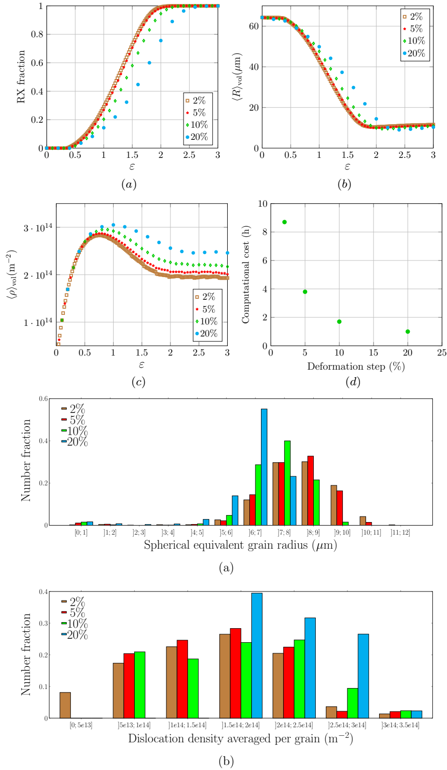
Fig. 3.8. Sensitivity of the deformation step on polycrystal results. The simulated process is a channel-die compression at 1273K, at a strain rate of 0.01s^{-1} during 300s. The mean values are weighted by grain volume for a better representativeness of the curves at the onset of recrystallization.
