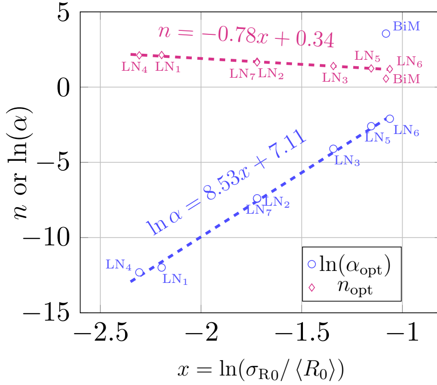
Fig. 2.15. Optimized values \alpha_{opt} and n_{opt} obtained by inverse analysis from the full field simulation results and linear relationships between the set of parameters (\ln(\alpha); n) and the ratio \ln(\sigma_{R0} / \langle R_0 \rangle) .
