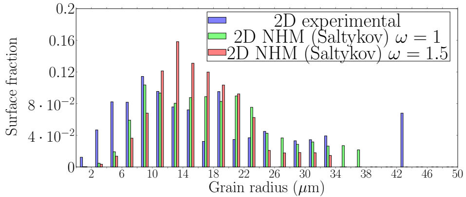
(c) T=1373\text{K} , \dot{\varepsilon}_{\text{VM}}=0.014\text{s}^{-1} , \varepsilon_{\text{VM}}=1.35 , X_{\text{expe}}=72.5\%
