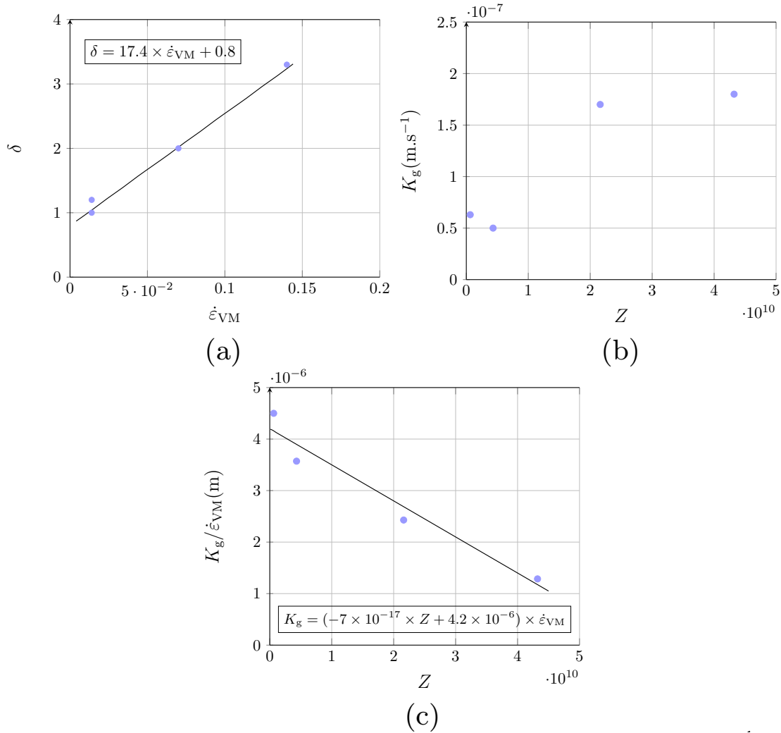
Fig. 5.27. Representation of (a) the \delta parameter as a function of strain rate, (b) the K_g parameter as a function of the Zener-Hollomon parameter and (c) the ratio K_g / \dot{\epsilon}_{\text{VM}} as a function of the Zener-Hollomon parameter.
