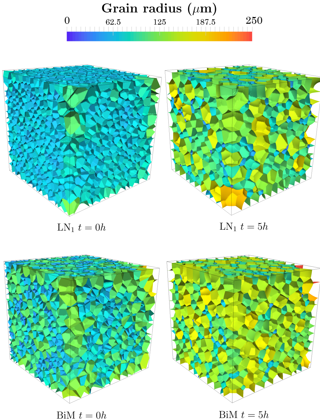
Fig. 2.7. Grain boundary networks at initial and final stages of the simulation for the \text{LN}_1 and BiM initial grain size distributions. The color code corresponds to the equivalent sphere radius of each grain.
