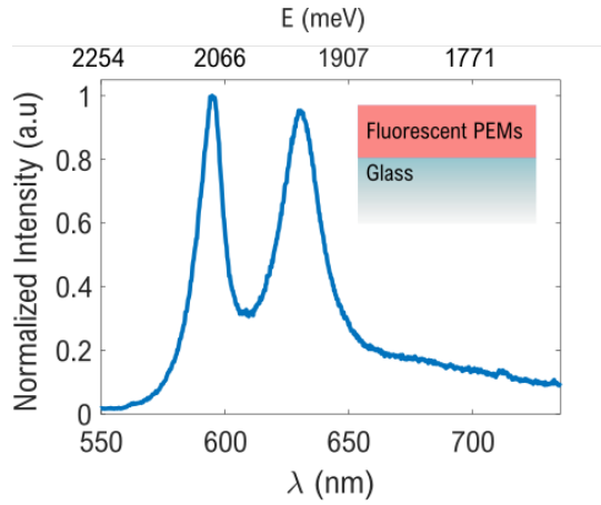
Figure 5.9 – Photoluminescence spectra of dye-1 and dye-2 on glass. Regions containing dye-1 and dye-2 are patterned following the same scheme as the one described in the previous section. The used deposition process is the same as for the one described in the previous section, but without the silver layer. The illumination consists of a wide-field laser excitation beam with a diameter of \varnothing = 50 \mu\text{m} . The normalized spectrum shows the dyes' emission with maximal values that have almost the same intensity despite the different number of layers of dye-1 and dye-2 deposited on the substrate. Also, we notice a long tail for wavelengths larger than 650 nm.
