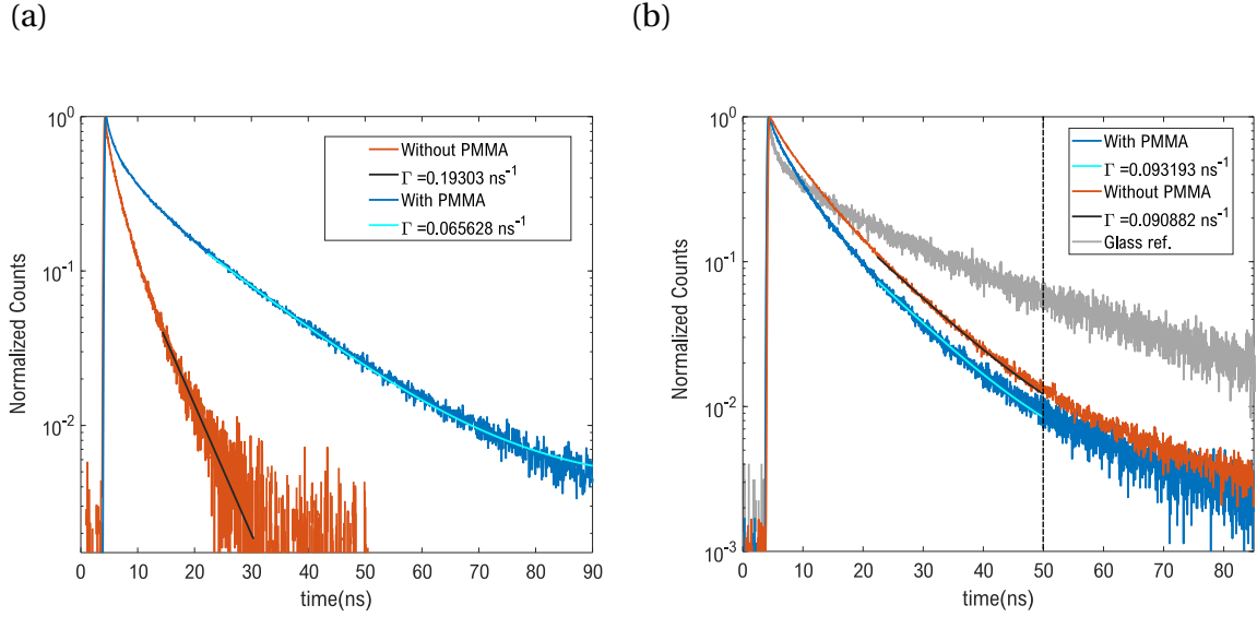
Figure B.2 – (a) Decay rate histograms for measurements of samples of diluted QDs spin-coated on top of a 70nm PVA spacer. The blue curve shows the histogram for a sample in which the QDs are embedded in PMMA, while in the sample corresponding to the red curve there is no polymer matrix. (b) Same as (a) but with a concentration of QDs equal to the one used for samples RLP, RUP1 and RUP2. The decay rate histogram of diluted QDs on glass was added to observe how the curves converge to a similar exponential decay for times t > 50 \text{ ns} . We performed a single exponential convoluted with the IRF fit in both curves to quantify the difference between decay rates. The values of Gamma resulting from the fit are reported in the legend of the figure.
