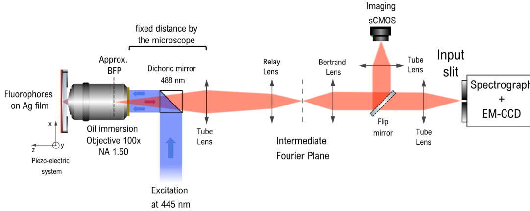
Figure 3.10 – Scheme of the setup and ray-tracing to perform spectroscopy of the reciprocal-space image of fluorescent samples. The incoming laser excitation is focused on the sample which position is controlled by piezoelectric actuators. The emission is directed either to the input slit aperture of the spectrometer, or an sCMOS camera (Zyla 5.5, Andor) used as a reference. In the microscope used during this thesis, it is impossible by construction to place the BFP on the focal plane of the tube lens. Since the tube lens is inaccessible by design, the intermediate Fourier Plane is not at a noticeable position within the detection path. A Bertrand lens is inserted to conjugate the Intermediate Fourier Plane image with the detectors. For this configuration, only oil immersion objectives are used.
