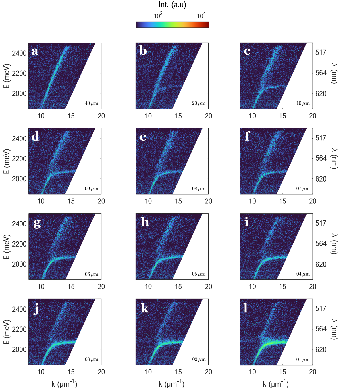
Figure A.2 – (a)-(l) Luminescence dispersion observed by focusing the laser at the center of the CPAs. The diameter is indicated in the lower right corner of the dispersion images.
