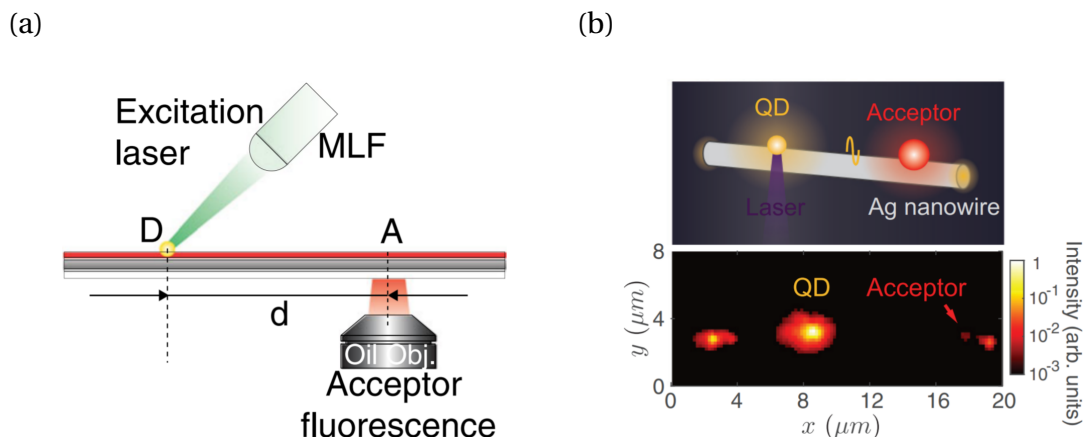
Figure 1.5 – (a) Scheme of the experimental setup to observe an energy transfer between a fluorescent bead (D, donor), excited by a micro-lensed fiber (MLF), and exciting the acceptors A in the surroundings through surface plasmons polaritons. Image taken from [20] (b) Top: Sketch of the experiment showing a single quantum dot and a fluorescent bead coupled to a silver nanowire. The quantum dot is excited and acts as the donor of the energy transfer process. Bottom: Electron multiplying CCD (EM-CCD) acquisition taken during the experiment, while the laser is focused on the QD. Bright spots are detected at the position of both emitters as well as both ends of the nanowire. Image taken from [21].
