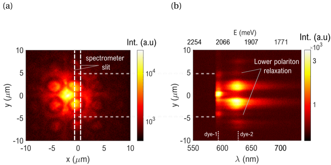
Figure 5.15 – Photoluminescence under a focused 532 nm laser excitation in the 0^\circ configuration. The quality of the dielectric film has optimal properties for the hybrid modes to propagate through this region of the sample. For the spatial distribution of the spectrum, we performed a non-local measurement for which the center of the spectrometer slit is indicated with white dashed lines. b) Corresponding spectral distribution of the PL along the y axis. We observe the emission of dye-1 excited at the same position of the excitation and the strong luminescence from the closest disks. At y = \pm 5\mu\text{m} , we observe the radiative relaxation of the system through the LP at the wavelength of dye-2.
