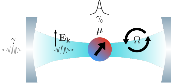
Figure 2.4 – Sketch of a molecule with dipolar moment \mu interacting with an optical cavity that has a resonance for \mathbf{E}_k . The strength of the coupling is given by \Omega .
