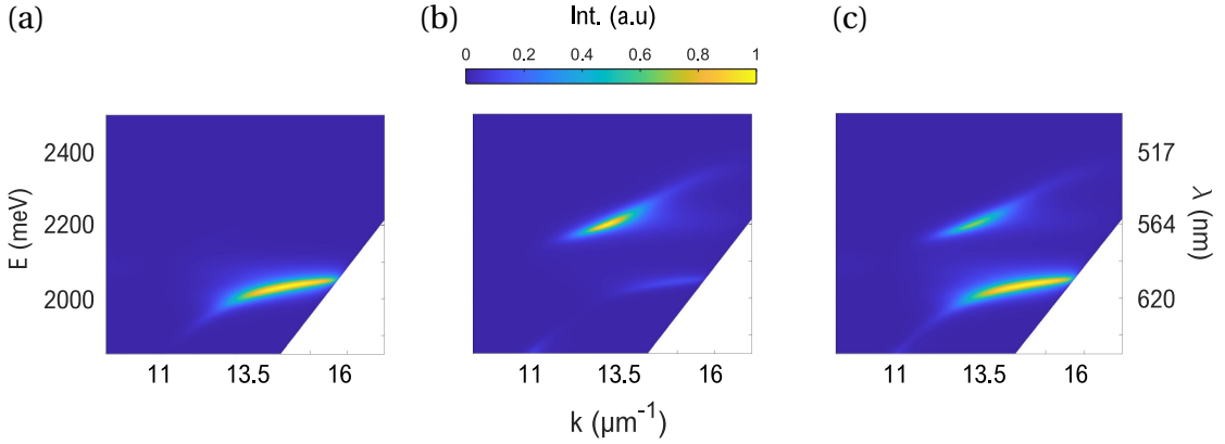
Figure 4.21 – Calculation of the emission pattern of a multilayered system composed by a glass substrate, a silver thin film h = 50\text{nm} , a layer of TDBC J-aggregates h_1 = 18\text{nm} and a layer of QDs h_1 = 15\text{nm} with a emission at 2156\text{meV} . The method uses a Rigorous Coupled Wave Analysis (RCWA) algorithm with the Kirchhoff model described in the main text. The independent emission of the layers is shown in (a) for the J-aggregates and in (b) for the QDs layer. (c) shows the system intensity fitting the model to the experimental data shown in Figure 4.15(b). The obtained free parameter is \Delta\mu = 192\text{meV} .
